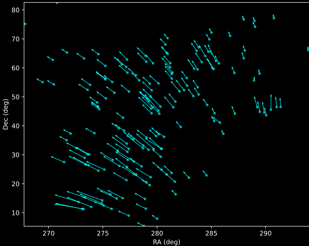
Gaia DR3 HDBSCAN 'Noise' (GD-1 Stream) (n=166)
