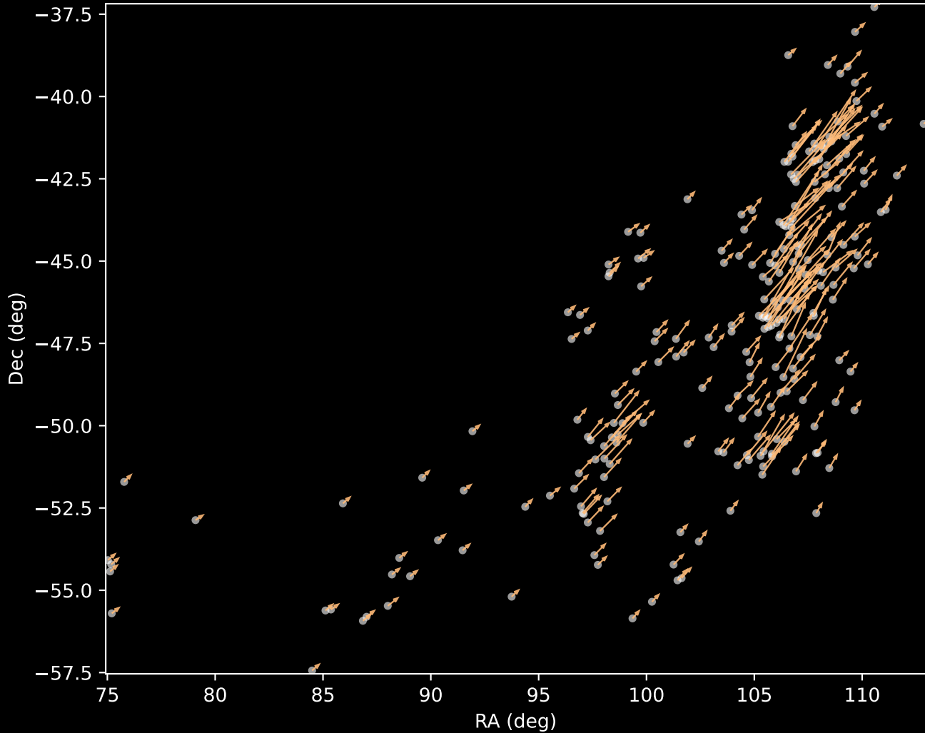
Gaia DR3 Cluster 3 Proper Motion Vectors (n=242)
