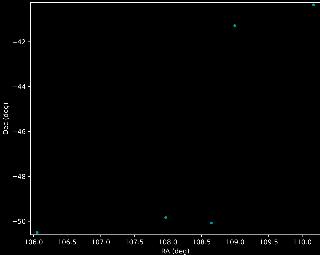
Gaia DR3 HDBSCAN 'Noise' (GD-1 Stream) (n=5)
