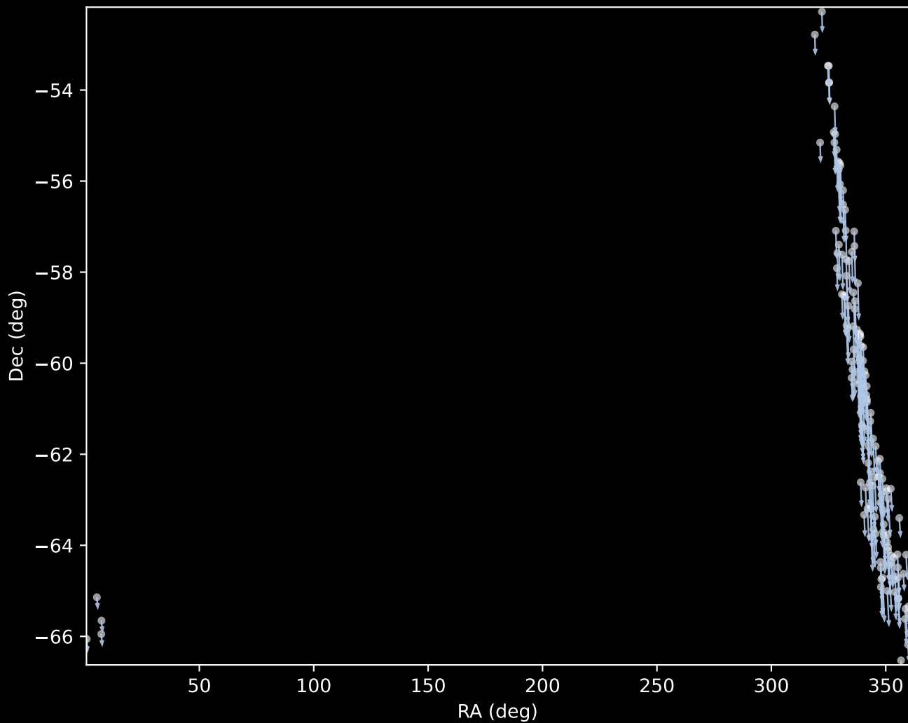
Gaia DR3 Cluster 1 Proper Motion Vectors (n=142)
