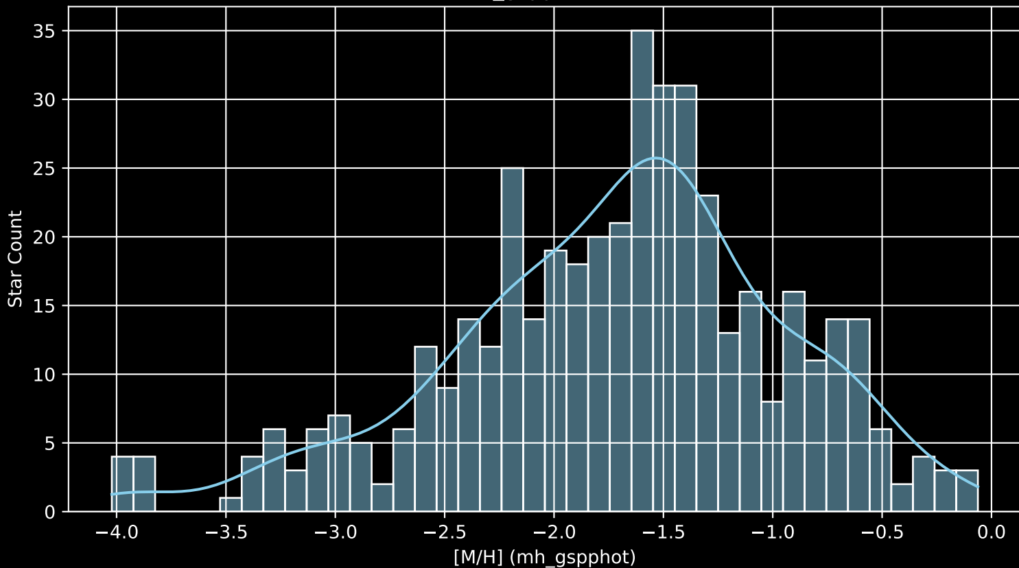
Gaia Stream: [Indus [M/H] (mh_gspphot) (n= 442)
