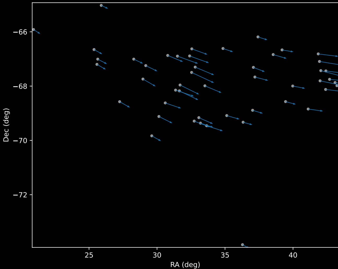
Gaia DR3 Cluster 0 Proper Motion Vectors (n=48)
