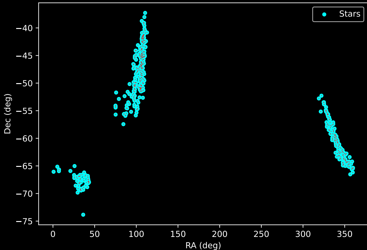
Gaia Stream: [Indus] Proper Motion Vectors for Gaia Star Field (n= 442)
