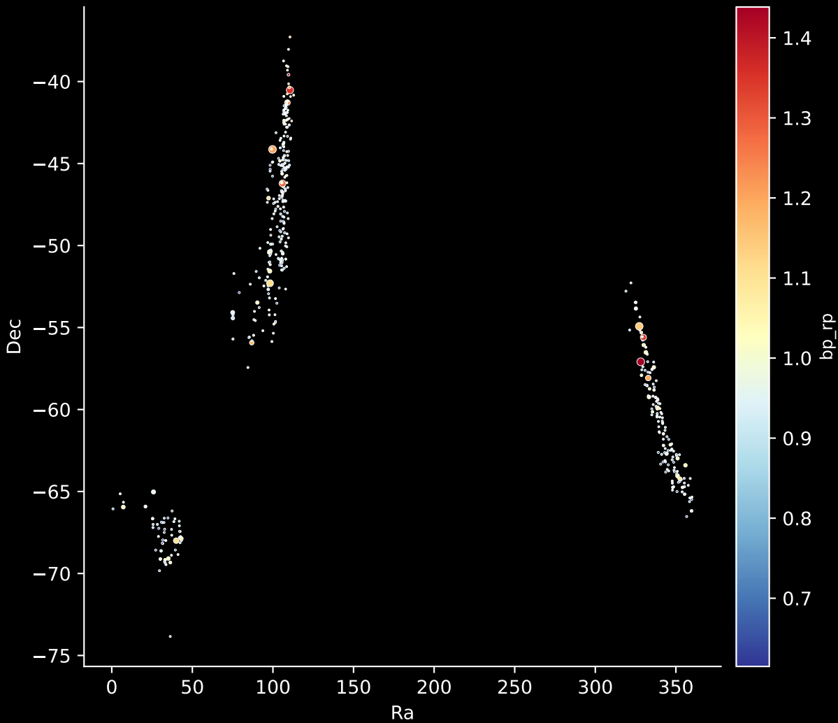
Gaia Stream: [Indus] Stars: 442
