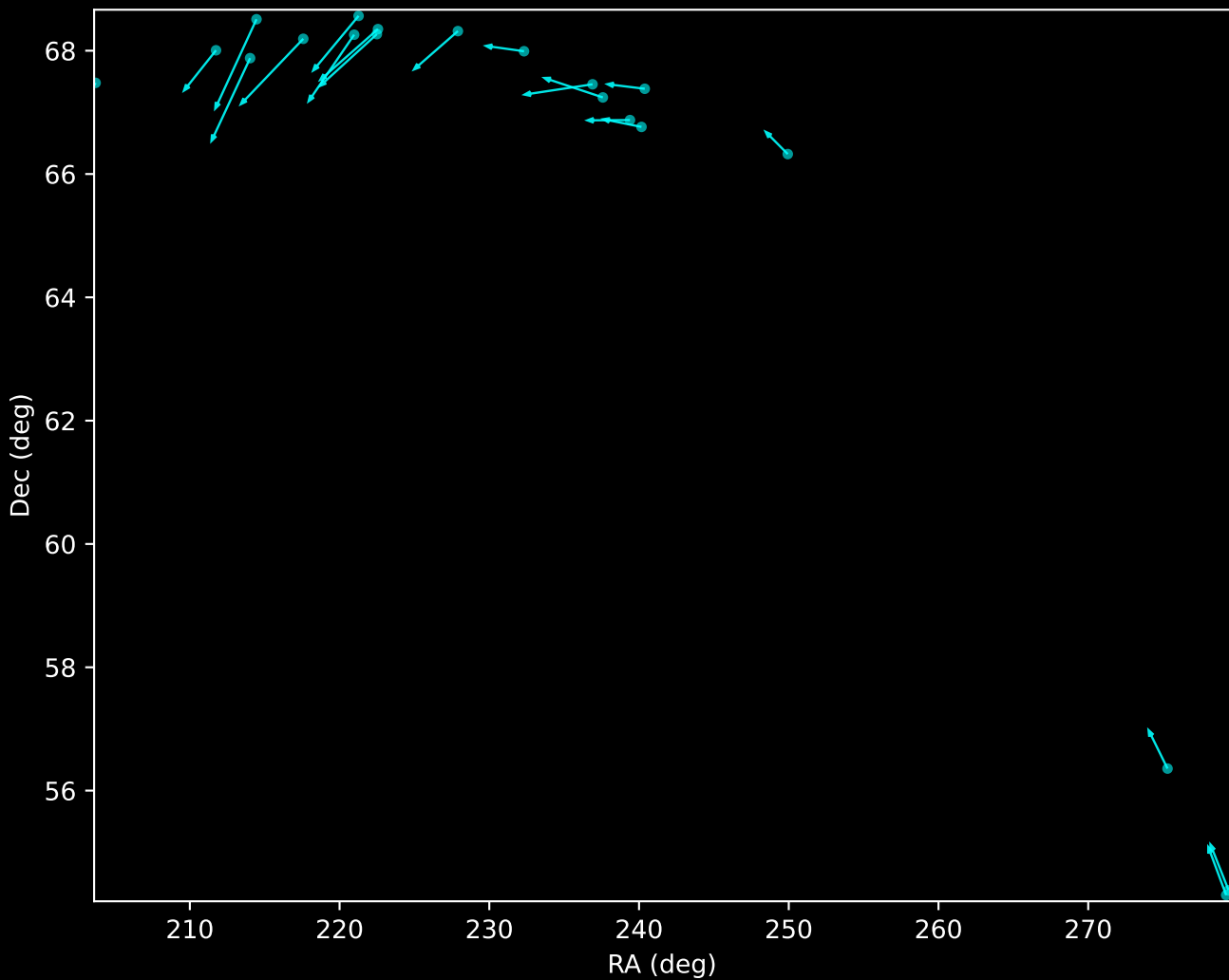
Gaia DR3 HDBSCAN 'Noise' (GD-1 Stream) (n=20)
