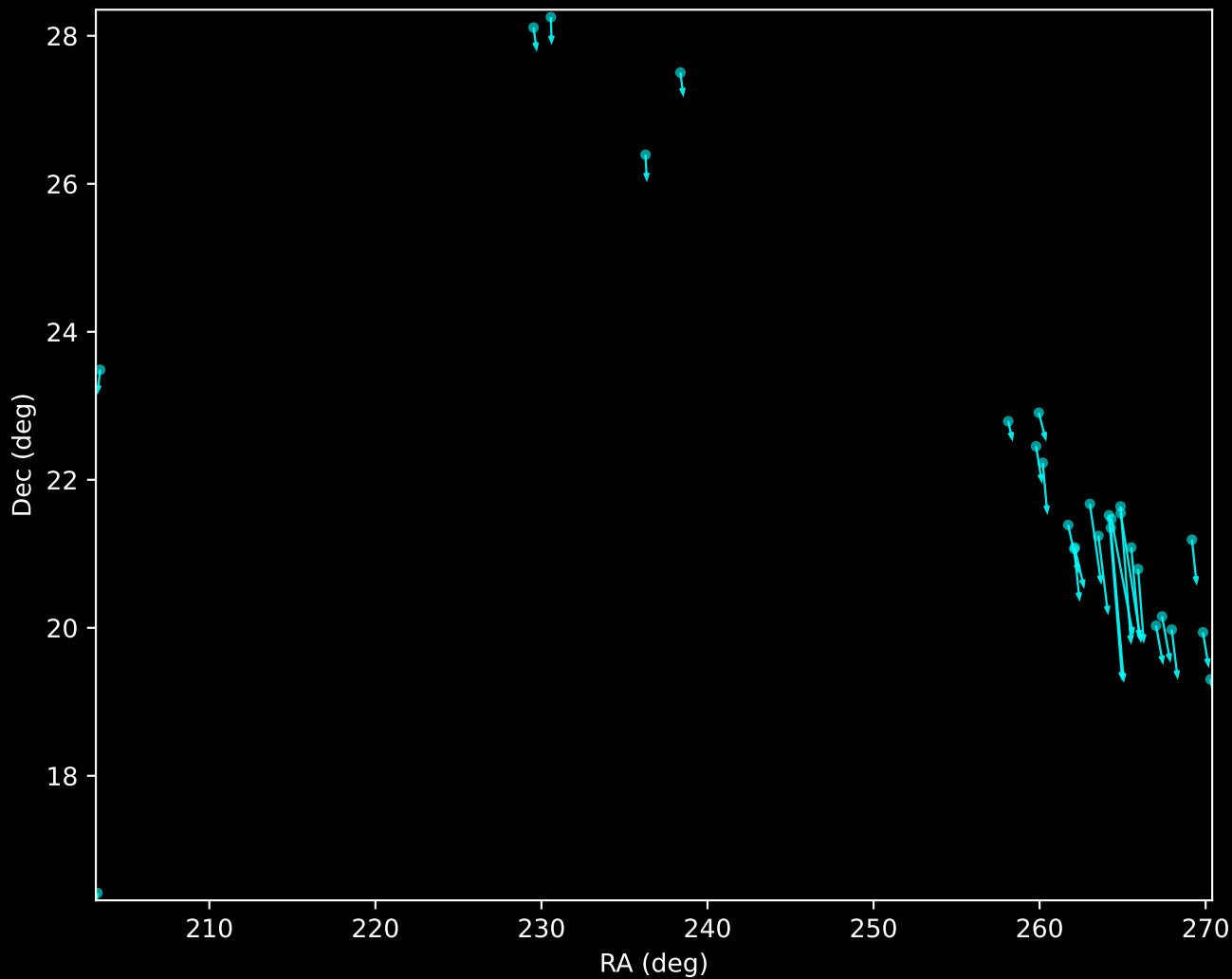
Gaia DR3 HDBSCAN 'Noise' (GD-1 Stream) (n=28)
