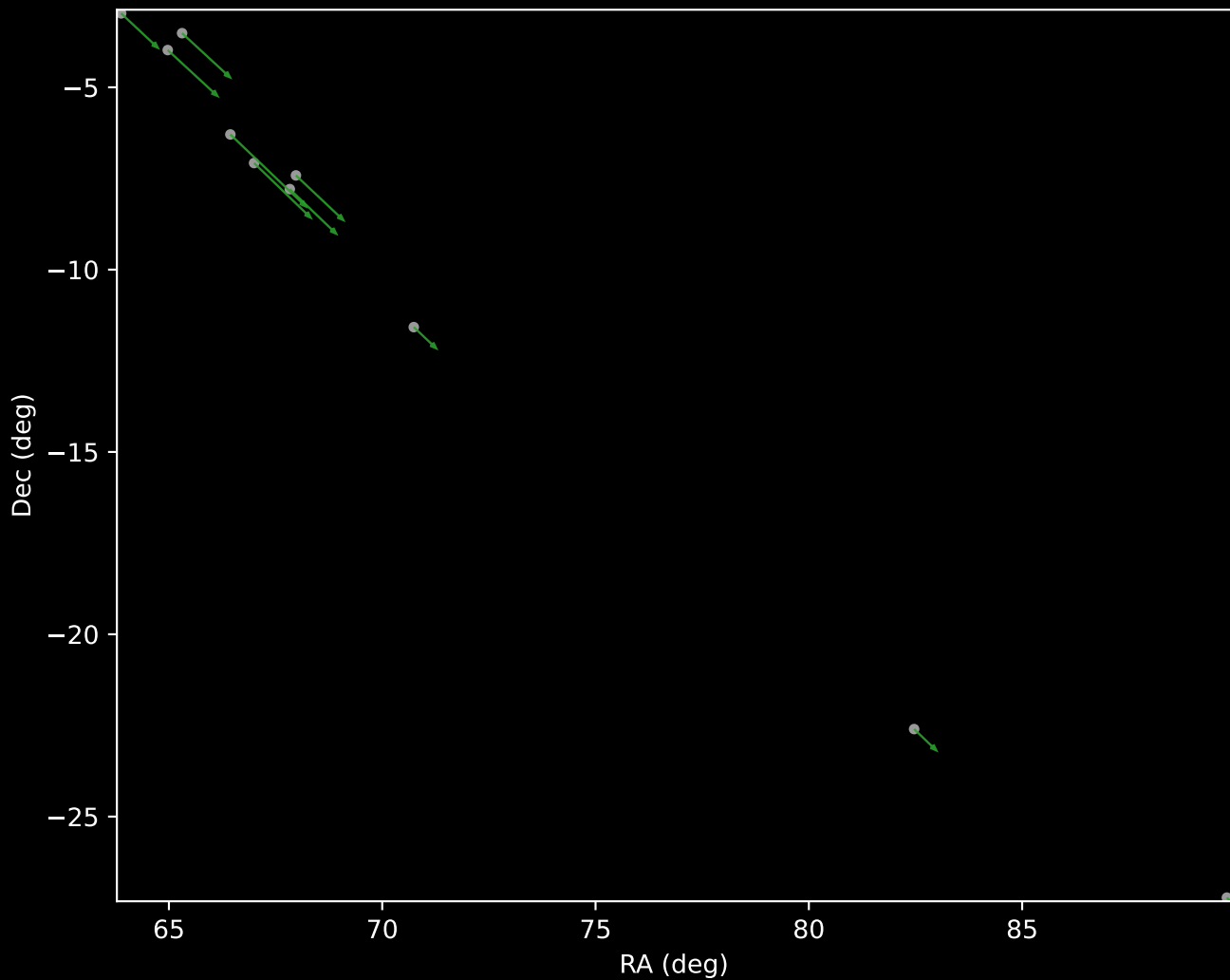
Gaia DR3 Cluster 4 Proper Motion Vectors (n=10)
