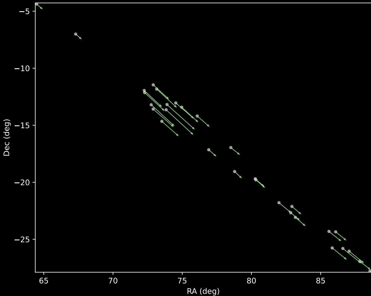
Gaia DR3 Cluster 5 Proper Motion Vectors (n=30)
