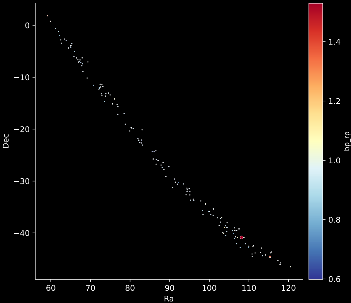
Gaia Stream: [Leiptr] Stars: 145
