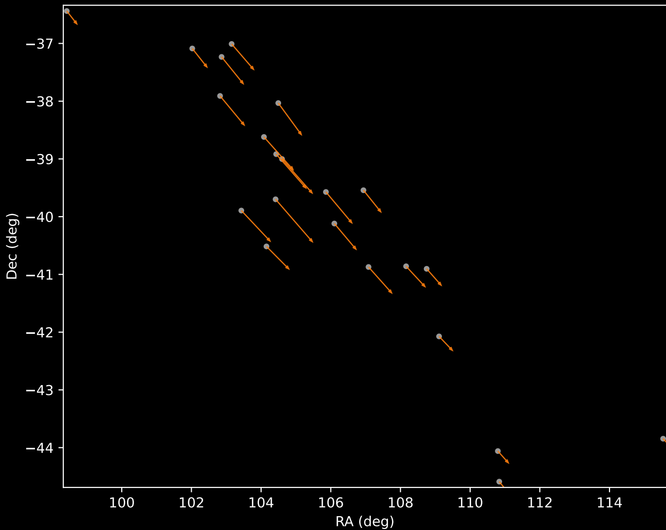
Gaia DR3 Cluster 2 Proper Motion Vectors (n=22)
