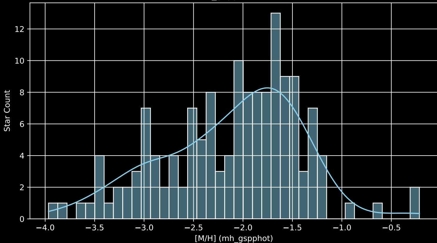
Gaia Stream: [Leiptr [M/H] (mh_gspphot) (n= 145)
