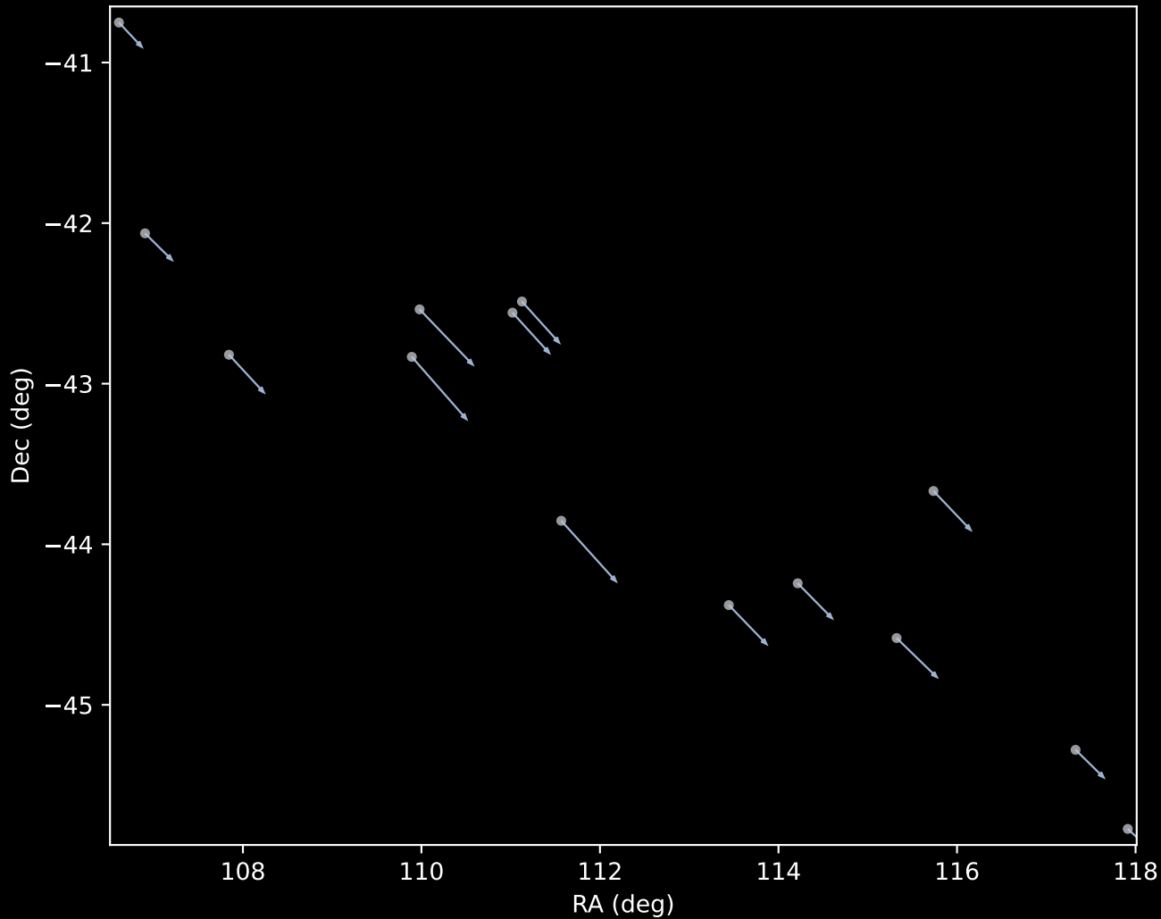
Gaia DR3 Cluster 1 Proper Motion Vectors (n=14)
