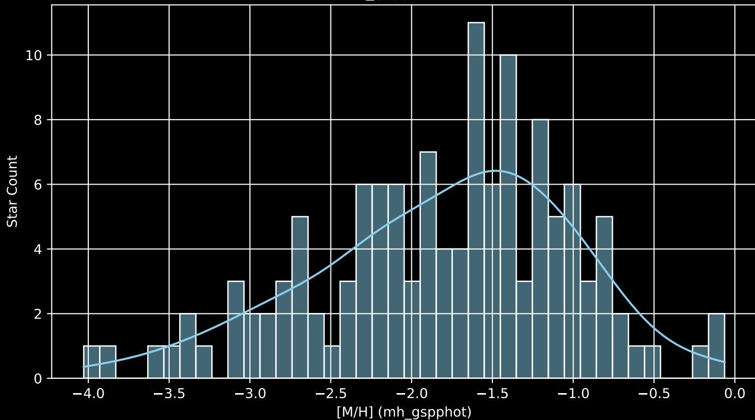
Gaia Stream: [M92 [M/H] (mh_gspphot) (n= 128)
