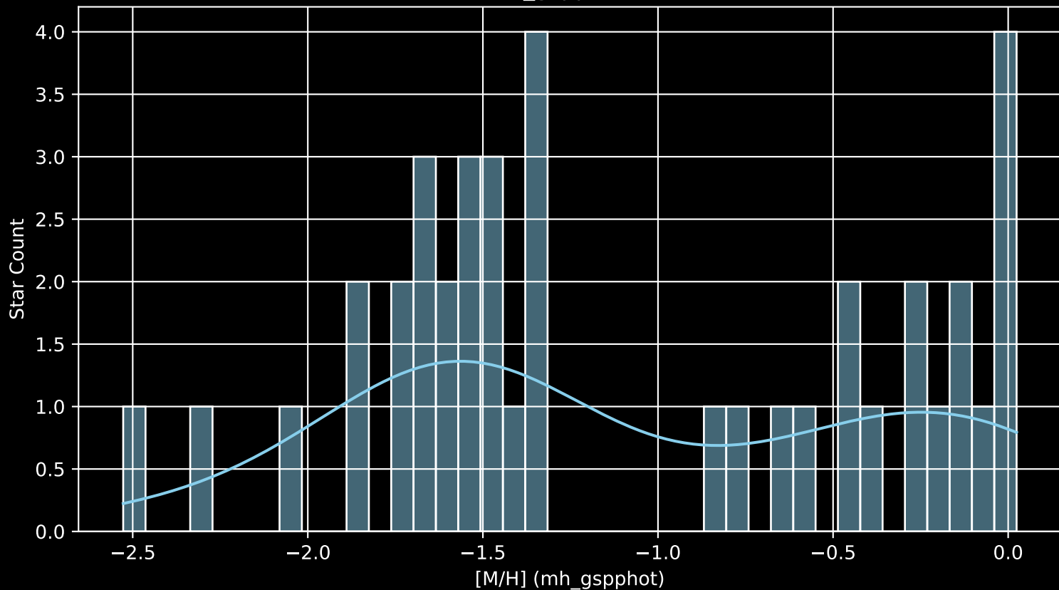
Gaia Stream: [NGC1851 [M/H] (mh_gspphot) (n= 40)
