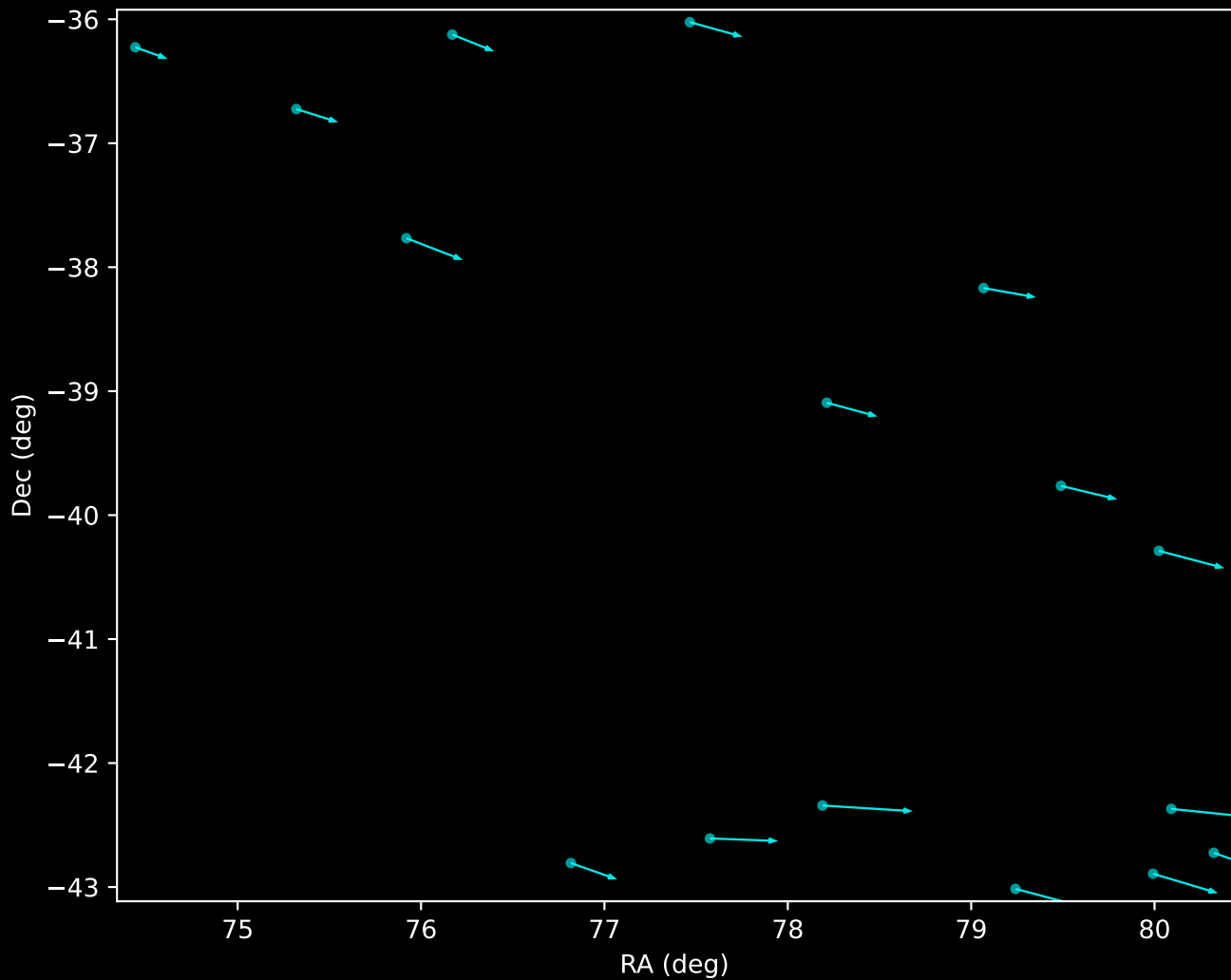
Gaia DR3 HDBSCAN 'Noise' (GD-1 Stream) (n=16)
