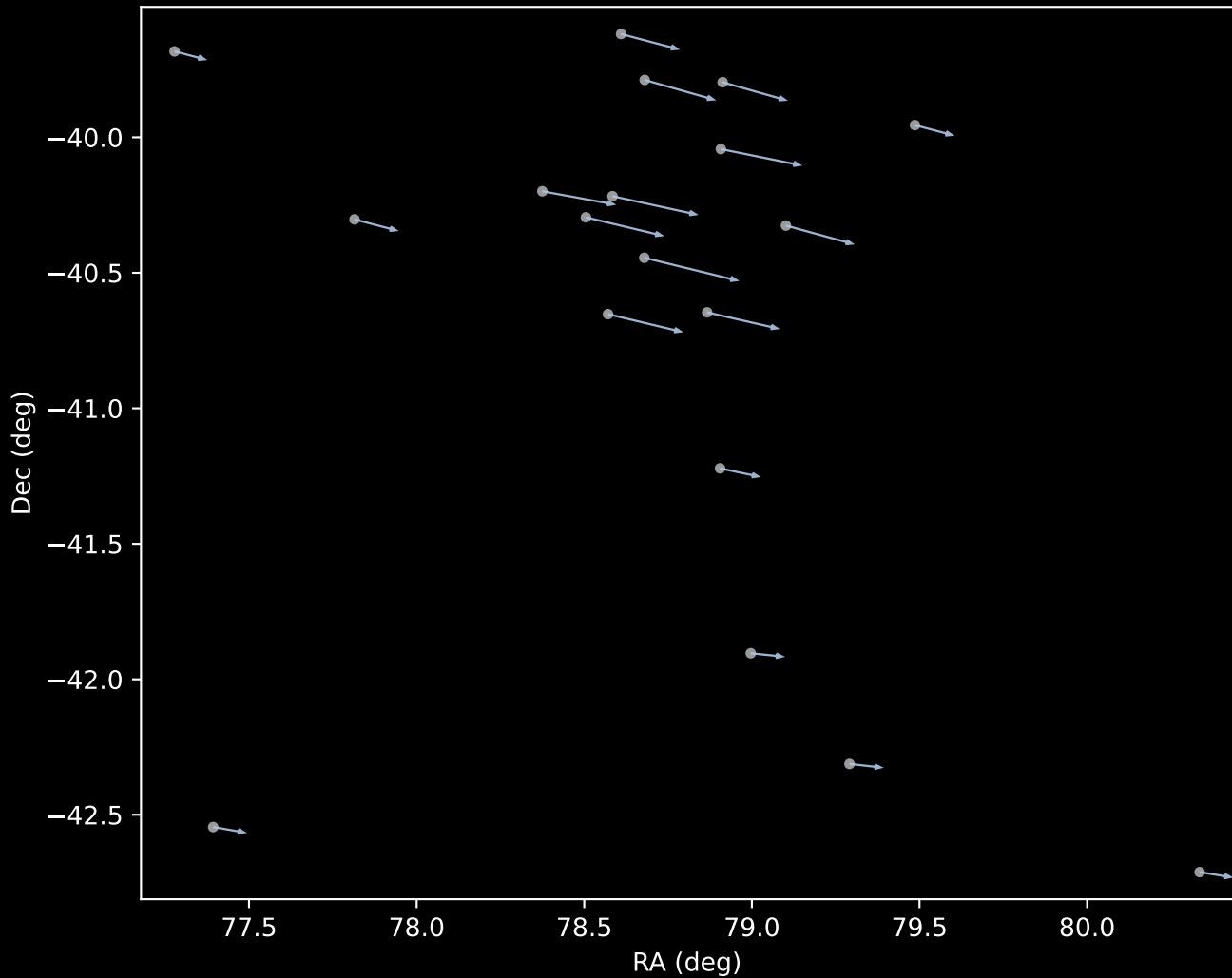
Gaia DR3 Cluster 1 Proper Motion Vectors (n=19)
