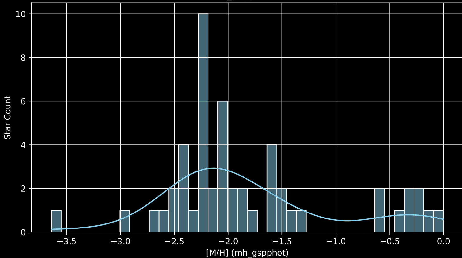
Gaia Stream: [NGC2808 [M/H] (mh_gspphot) (n= 51)
