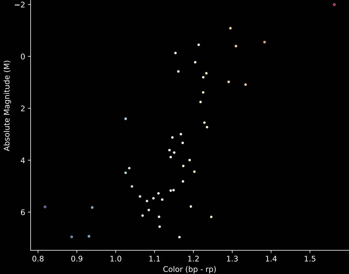
Gaia Stream: [NGC2808] Stream (n= 51) Hertzsprung-Russel Diagram
