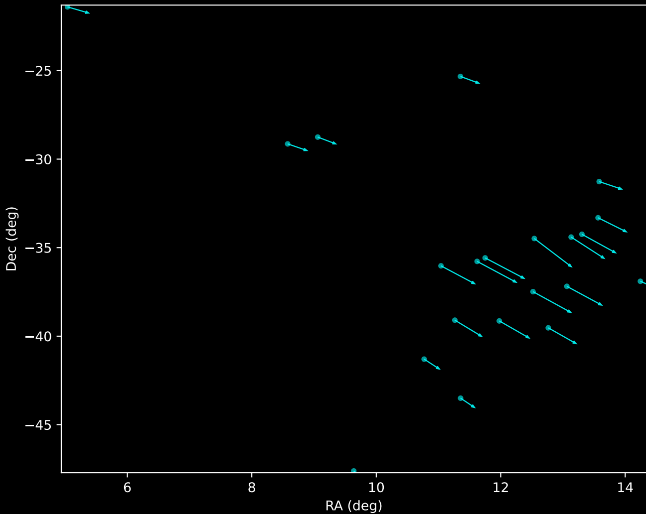
Gaia DR3 HDBSCAN 'Noise' (GD-1 Stream) (n=21)
