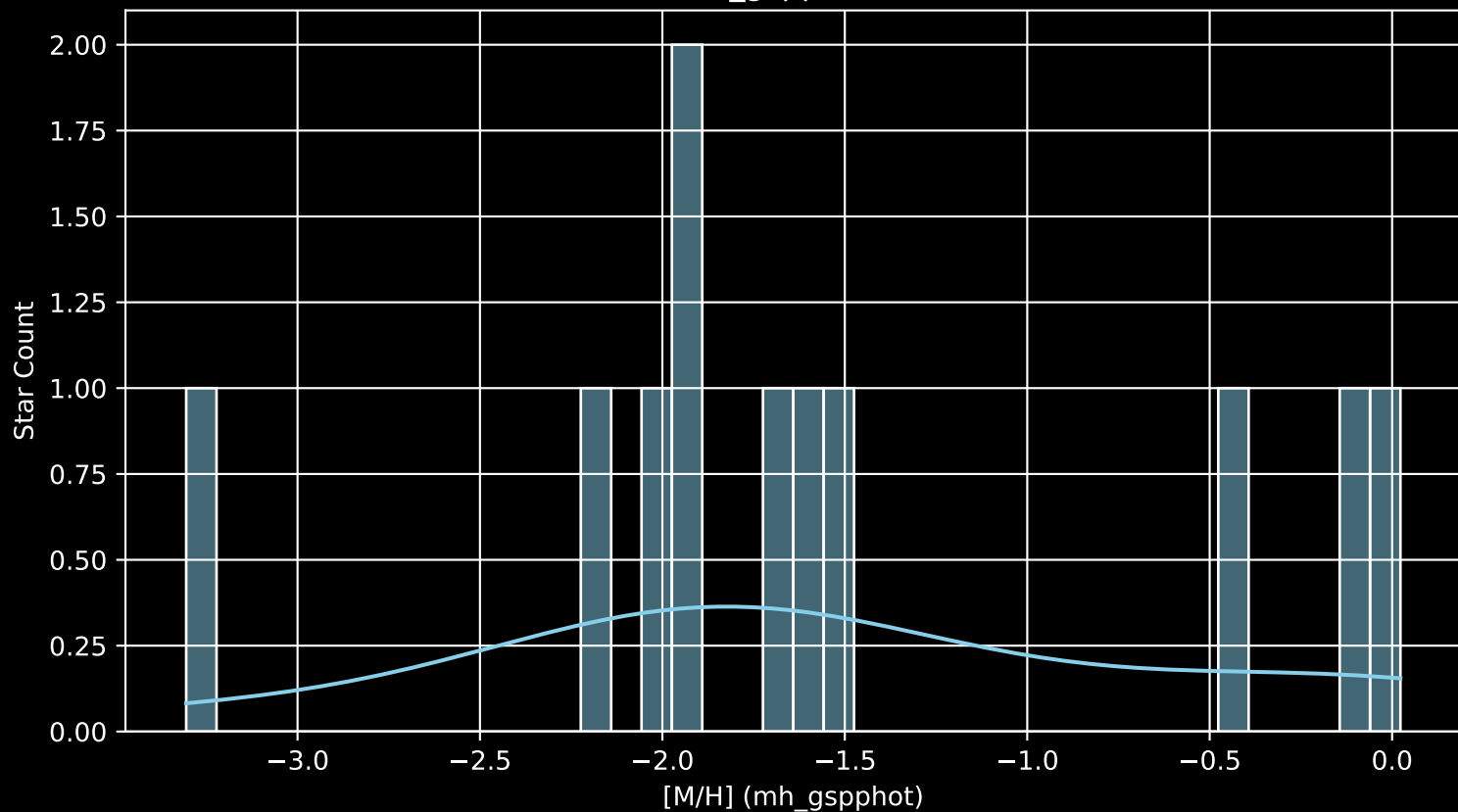
Gaia Stream: [NGC7492 [M/H] (mh_gspphot) (n= 11)
