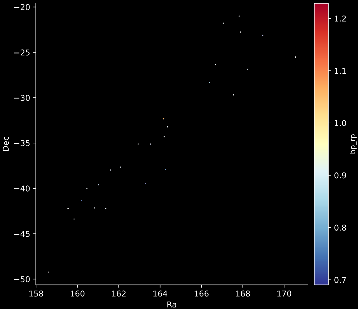
Gaia Stream: [New-13] Stars: 26
