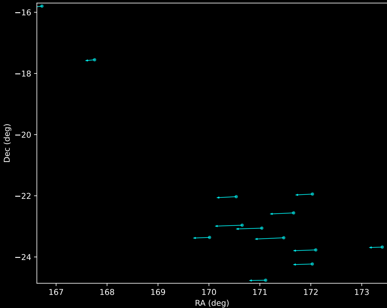
Gaia DR3 HDBSCAN 'Noise' (GD-1 Stream) (n=13)
