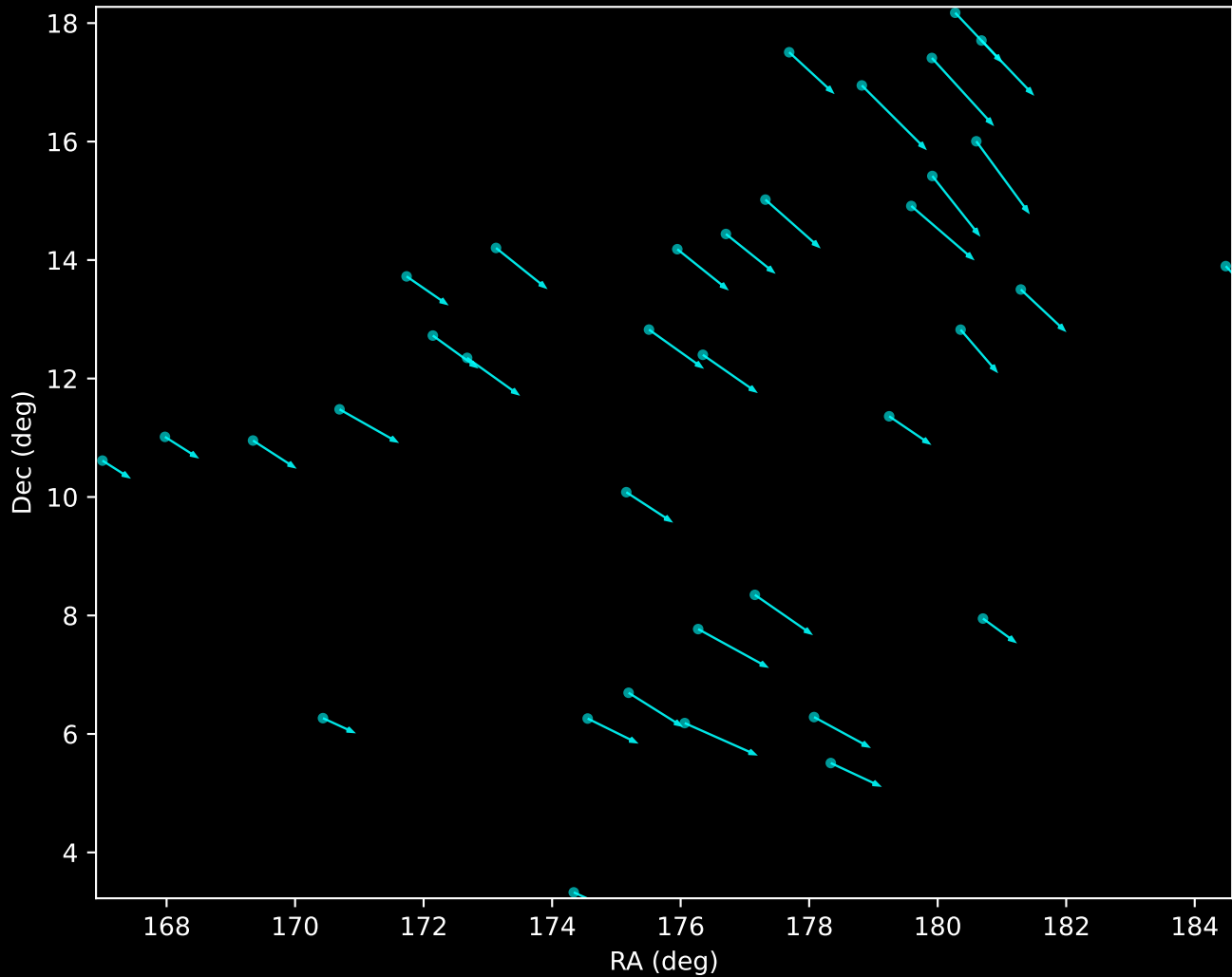
Gaia DR3 HDBSCAN 'Noise' (GD-1 Stream) (n=36)
