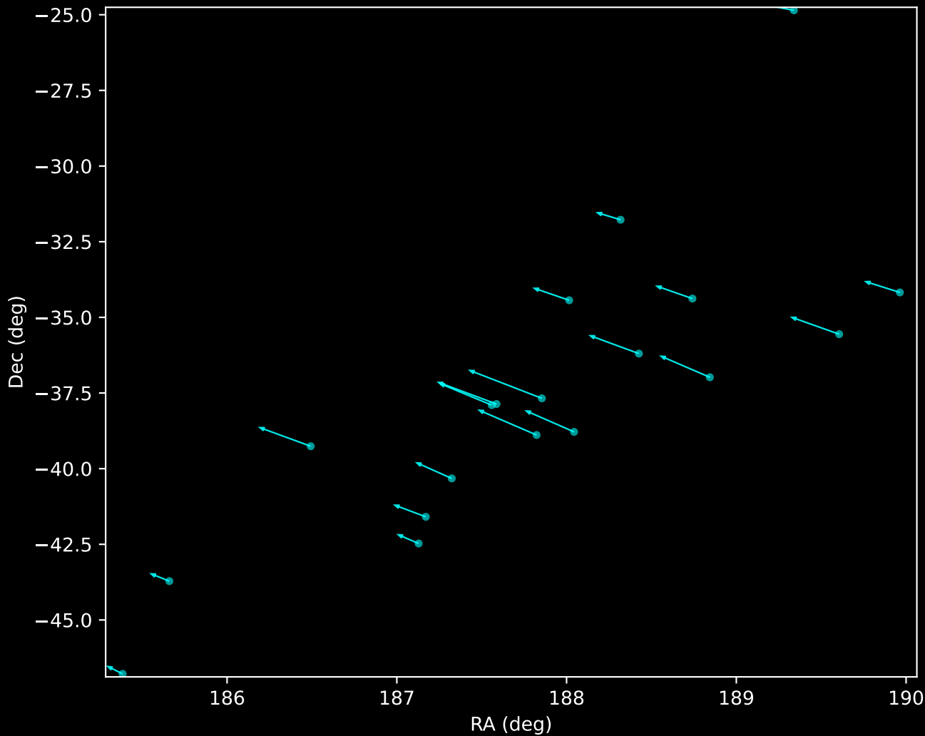
Gaia DR3 HDBSCAN 'Noise' (GD-1 Stream) (n=19)
