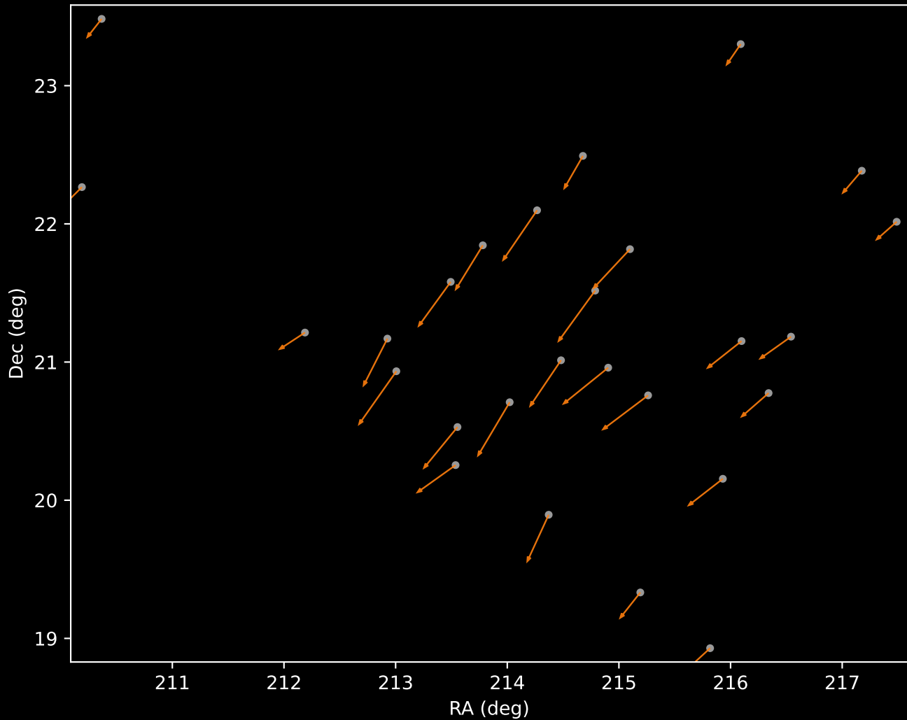
Gaia DR3 Cluster 2 Proper Motion Vectors (n=27)
