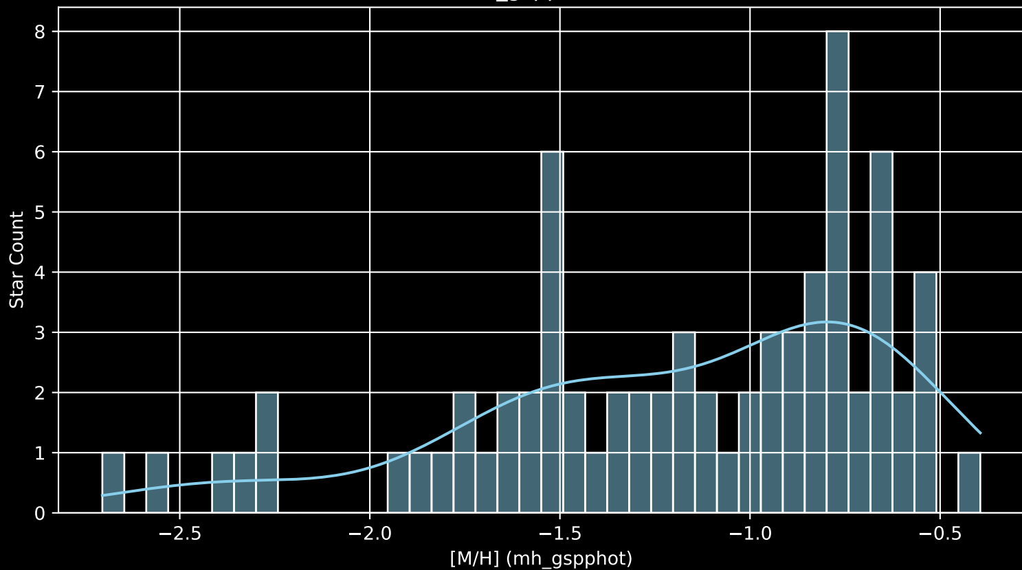
Gaia Stream: [New-18 [M/H] (mh_gspphot) (n= 72)
