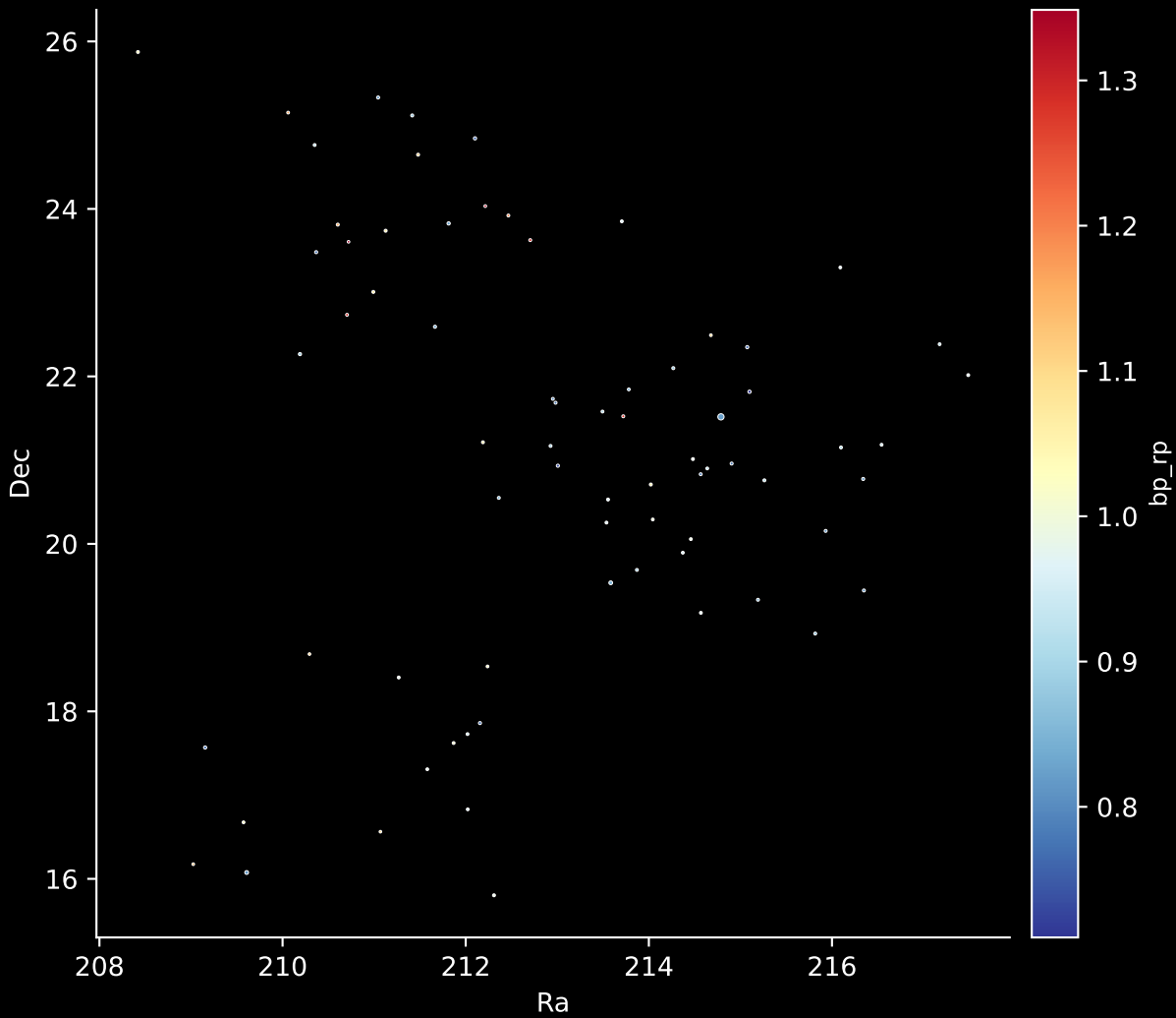
Gaia Stream: [New-18] Stars: 72
