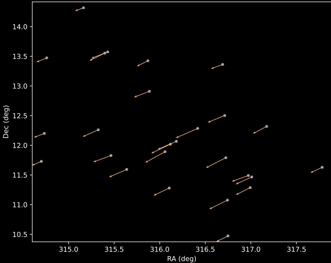
Gaia DR3 Cluster 23 Proper Motion Vectors (n=26)
