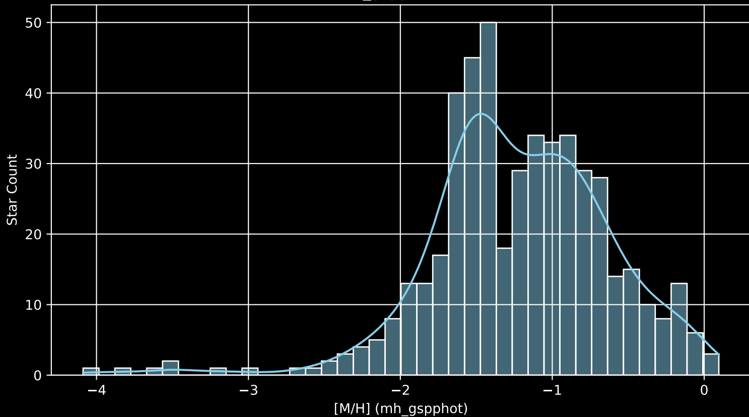
Gaia Stream: [New-21 [M/H] (mh_gspphot) (n= 483)
