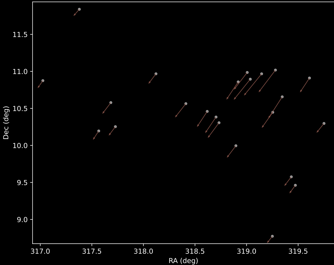
Gaia DR3 Cluster 10 Proper Motion Vectors (n=23)
