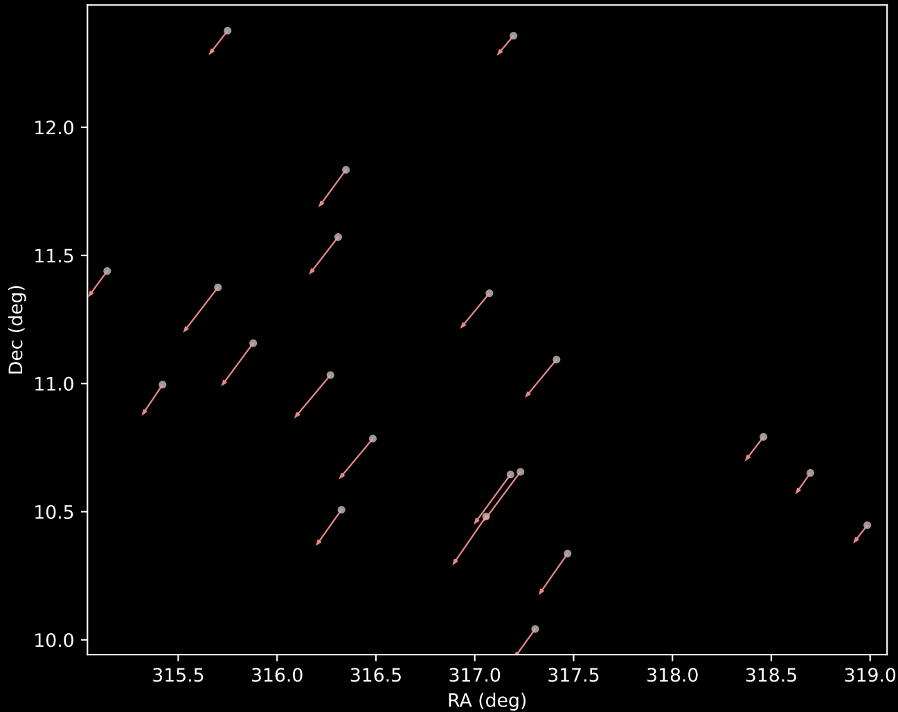
Gaia DR3 Cluster 27 Proper Motion Vectors (n=21)
