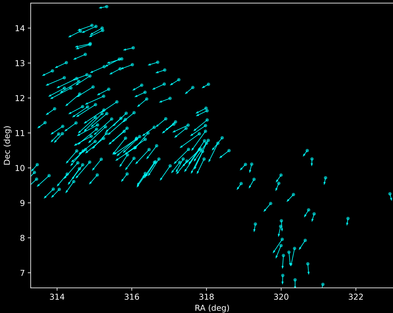
Gaia DR3 HDBSCAN 'Noise' (GD-1 Stream) (n=155)
