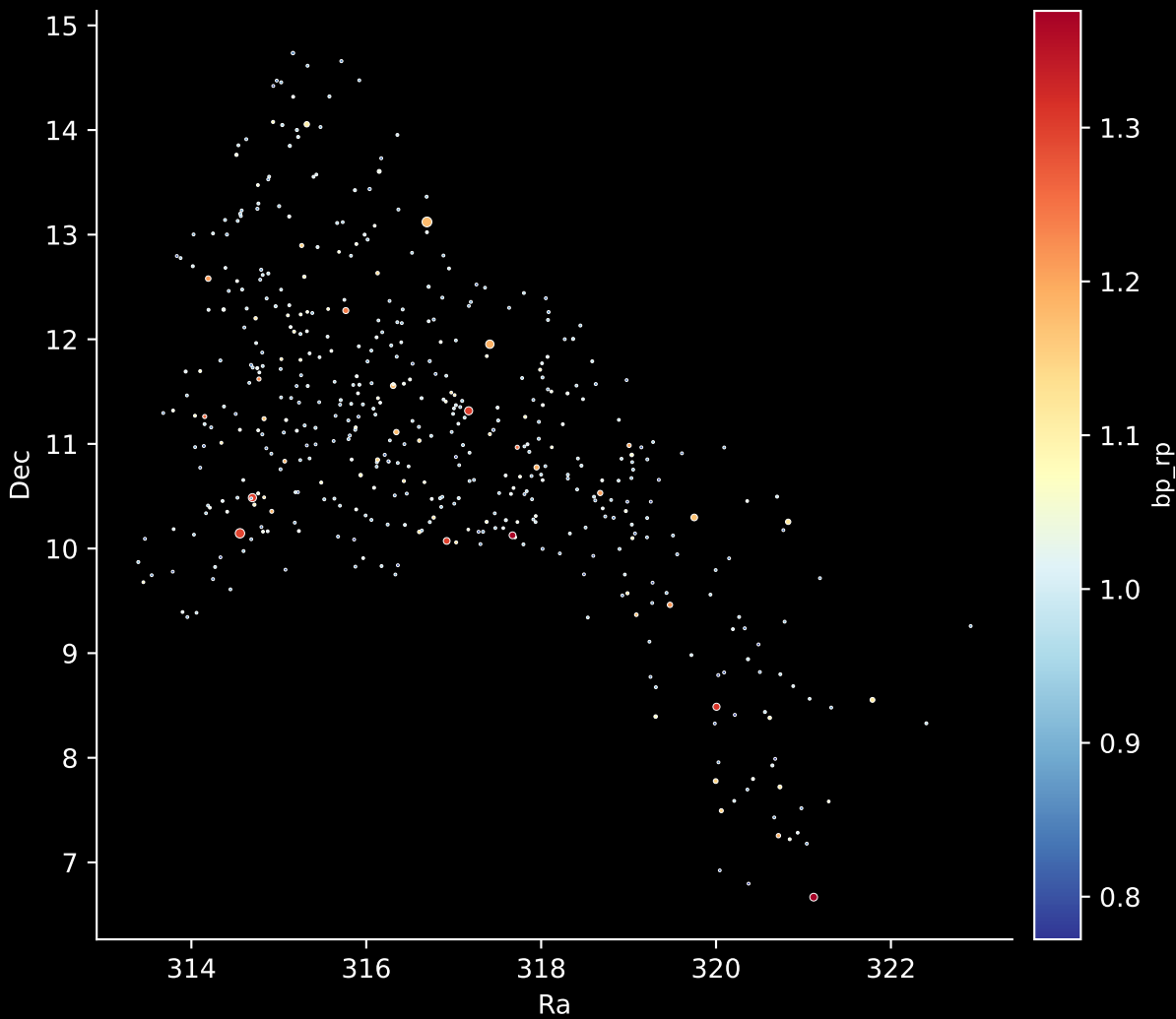
Gaia Stream: [New-21] Stars: 483
