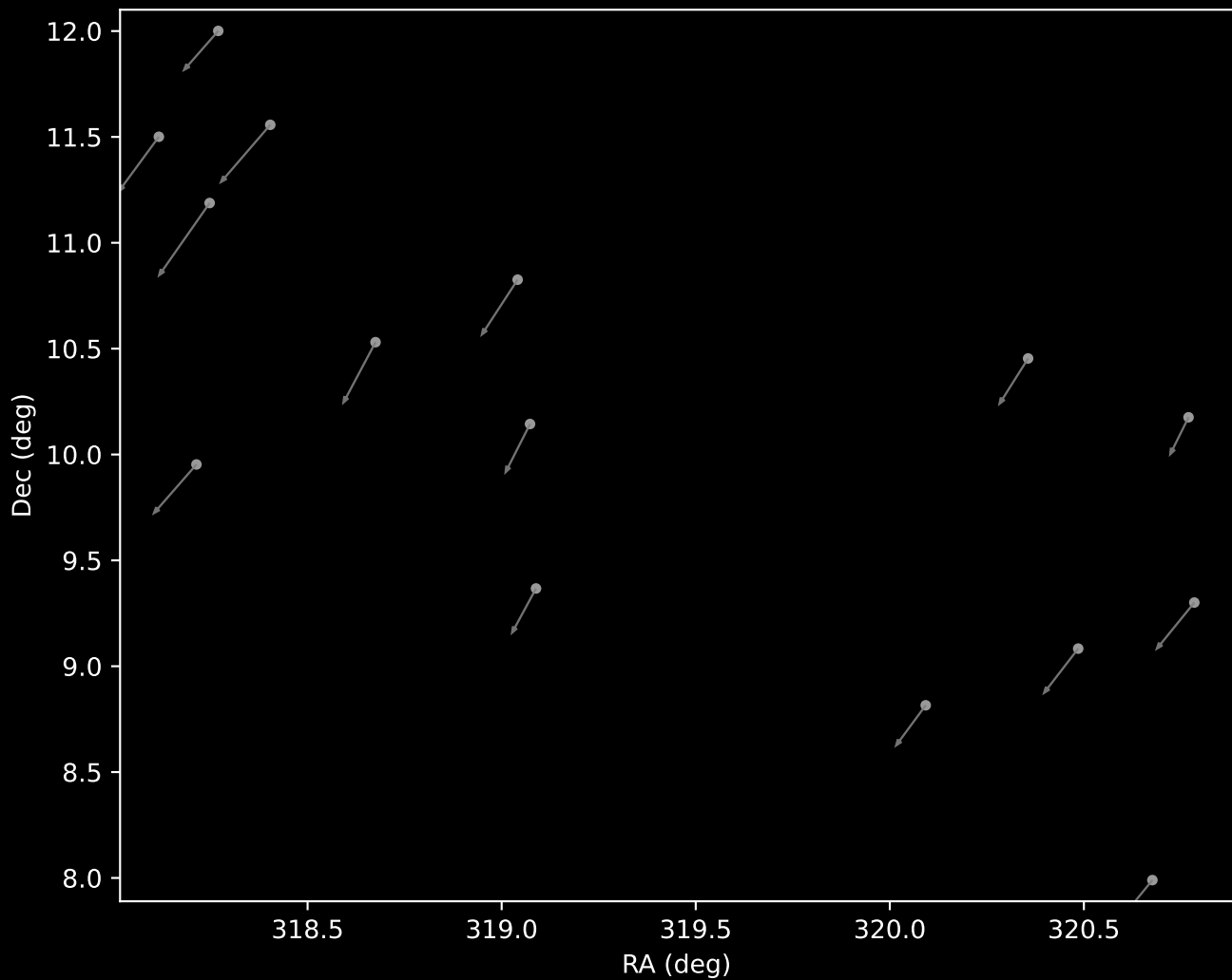
Gaia DR3 Cluster 14 Proper Motion Vectors (n=15)
