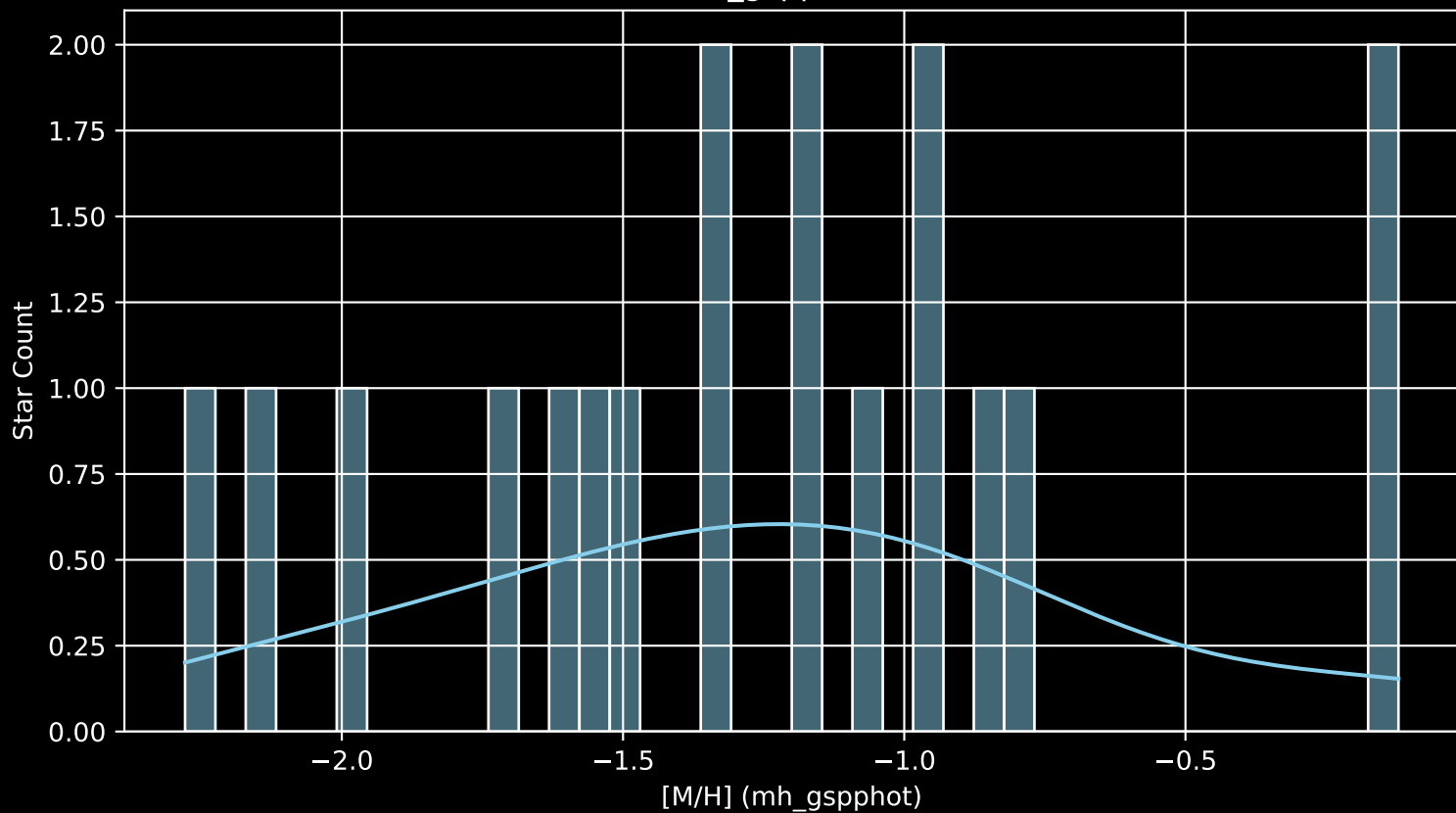
Gaia Stream: [New-22 [M/H] (mh_gspphot) (n= 18)
