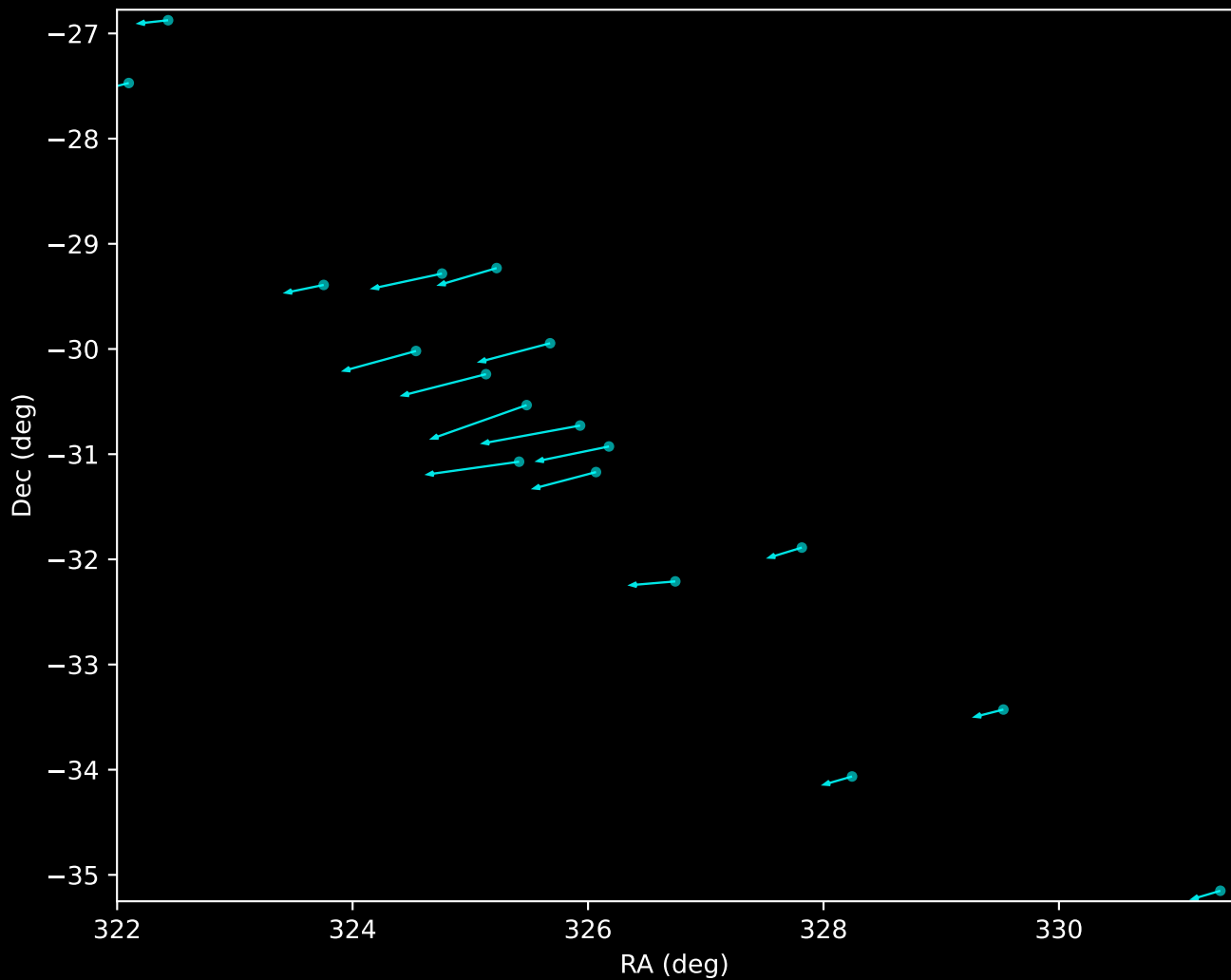
Gaia DR3 HDBSCAN 'Noise' (GD-1 Stream) (n=18)
