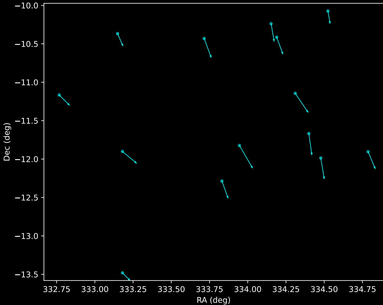
Gaia DR3 HDBSCAN 'Noise' (GD-1 Stream) (n=14)
