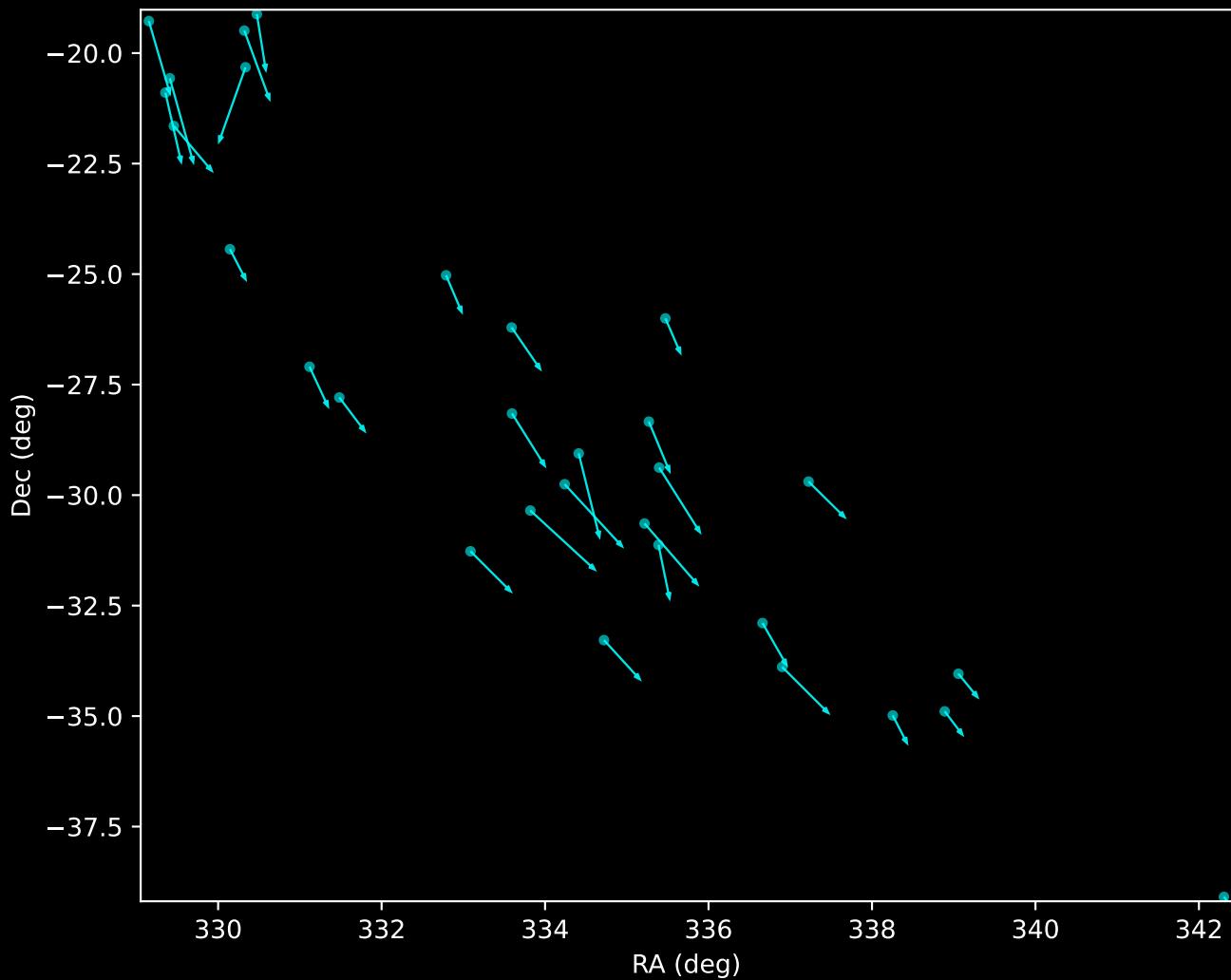
Gaia DR3 HDBSCAN 'Noise' (GD-1 Stream) (n=30)
