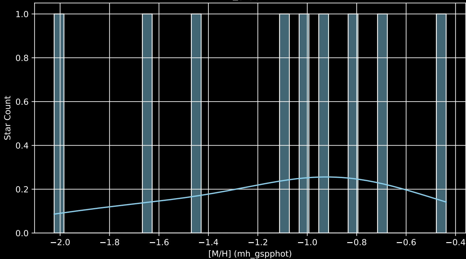
Gaia Stream: [New-5 [M/H] (mh_gspphot) (n= 9)
