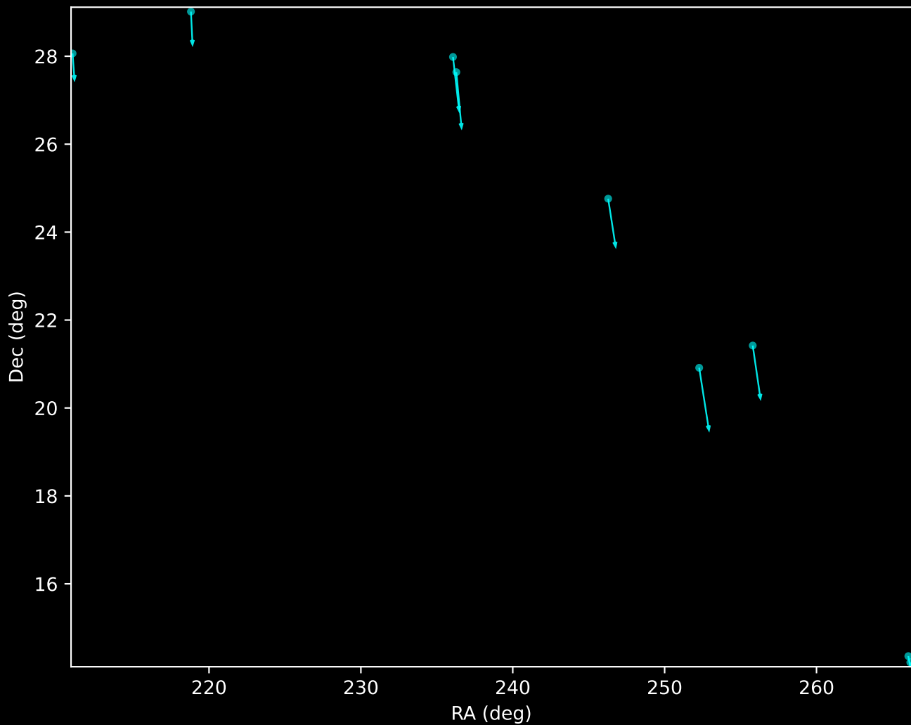
Gaia DR3 HDBSCAN 'Noise' (GD-1 Stream) (n=9)
