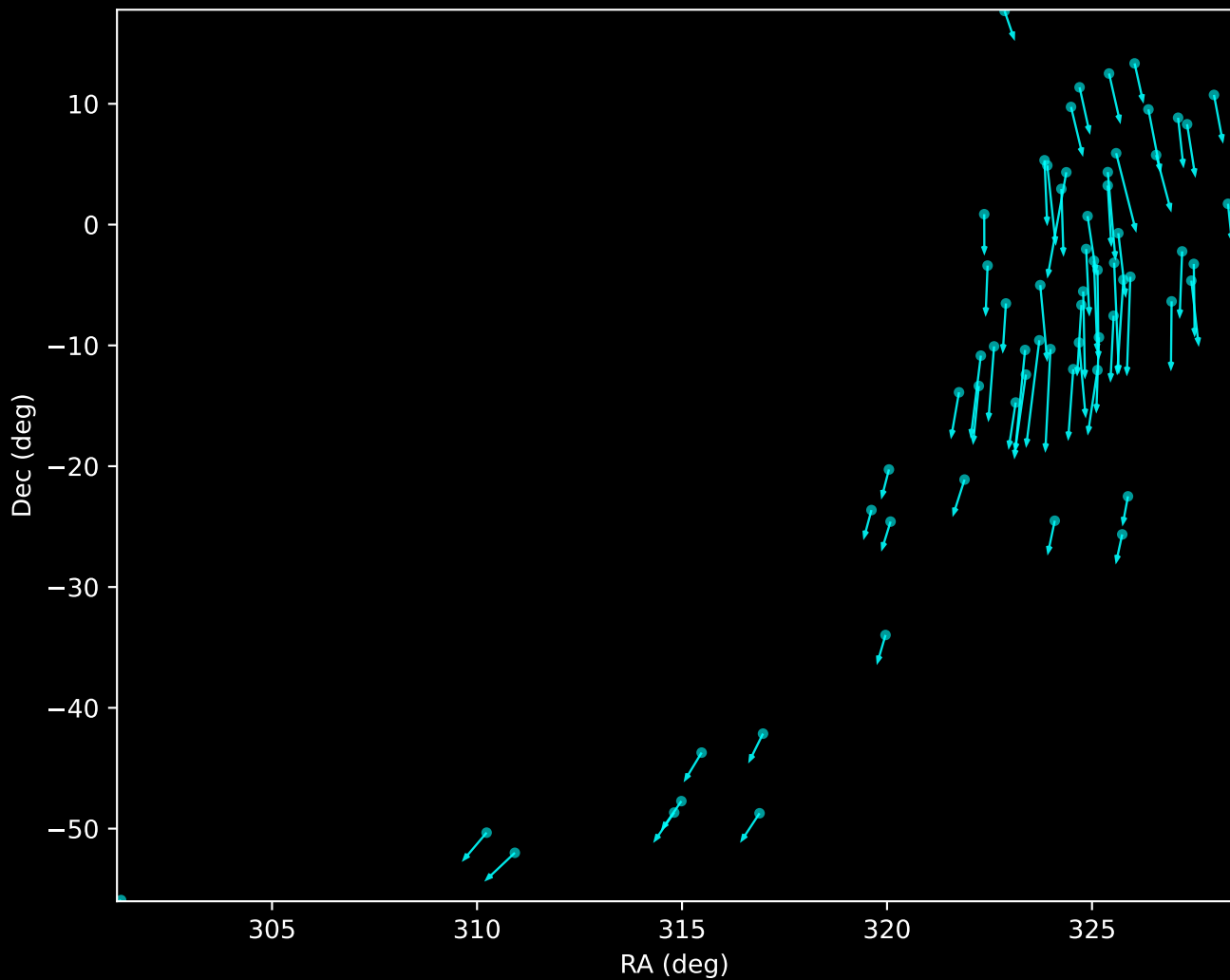
Gaia DR3 HDBSCAN 'Noise' (GD-1 Stream) (n=66)
