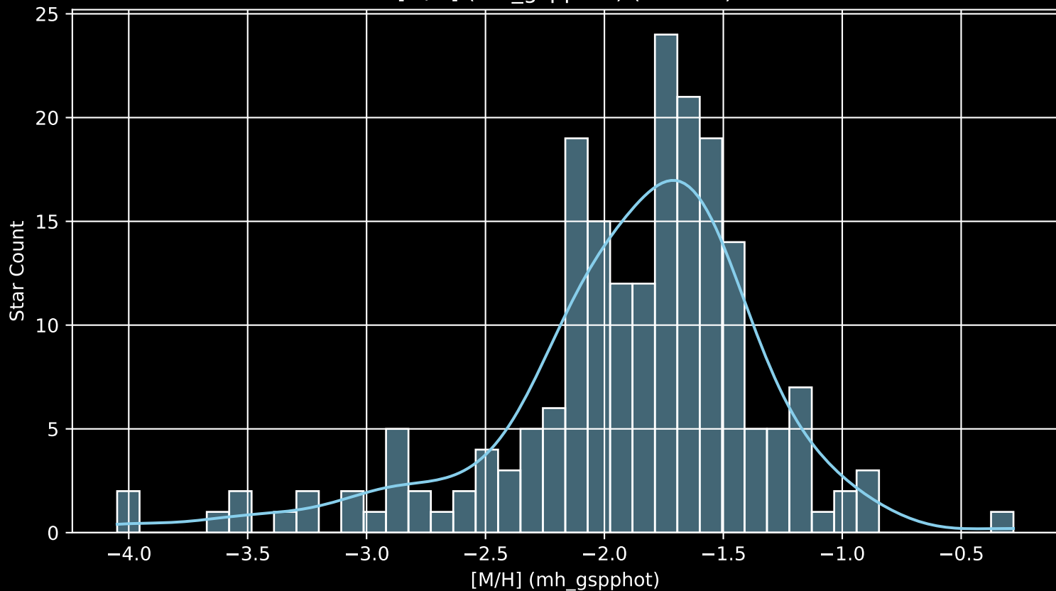
Gaia Stream: [Slidr [M/H] (mh_gspphot) (n= 199)
