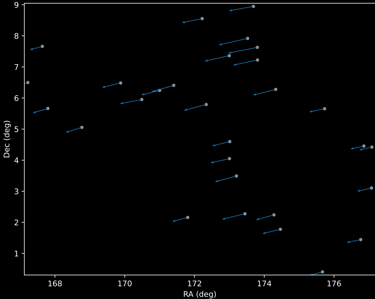
Gaia DR3 Cluster 0 Proper Motion Vectors (n=29)
