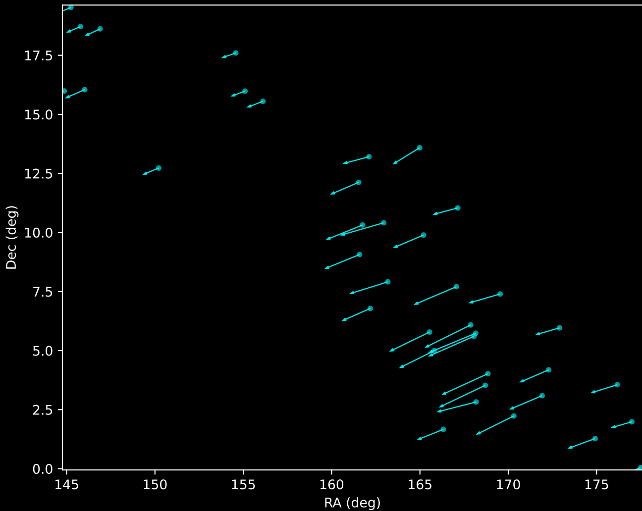
Gaia DR3 HDBSCAN 'Noise' (GD-1 Stream) (n=38)
