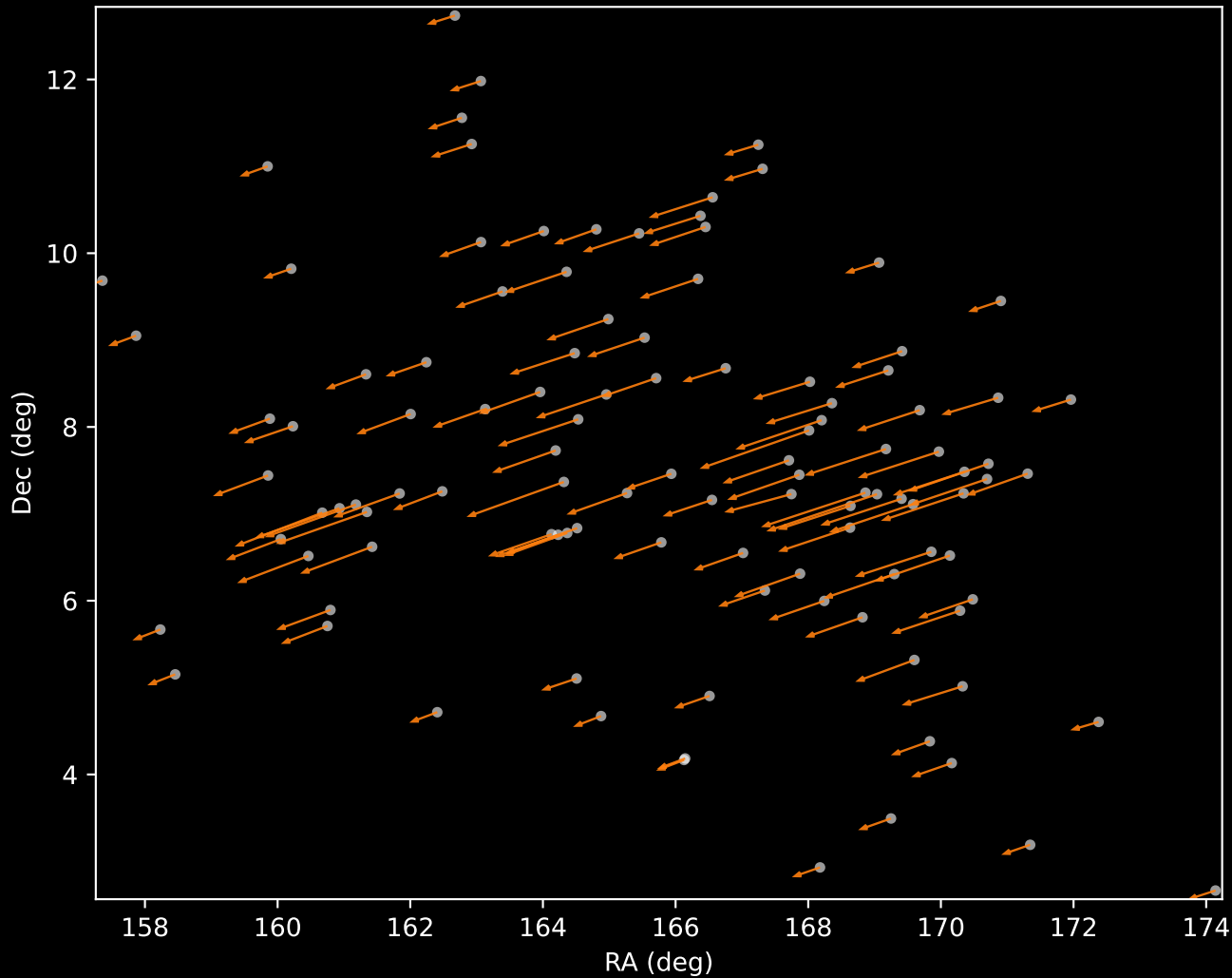
Gaia DR3 Cluster 2 Proper Motion Vectors (n=110)
