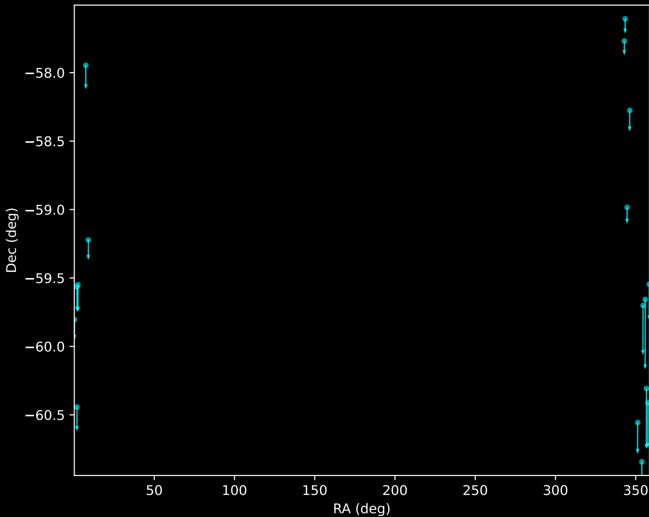
Gaia DR3 HDBSCAN 'Noise' (GD-1 Stream) (n=17)
