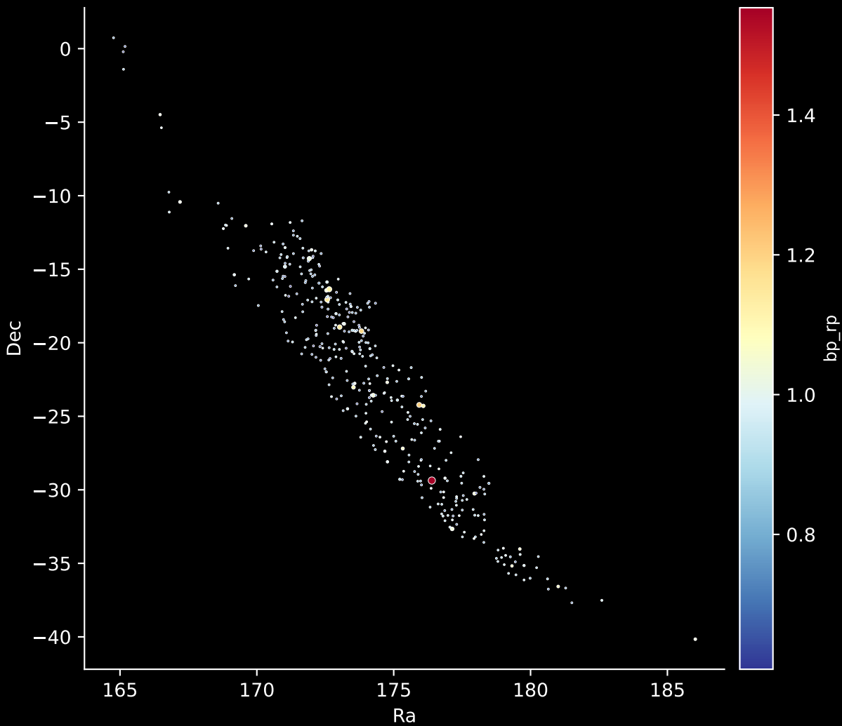
Gaia Stream: [Ylgr] Stars: 371
