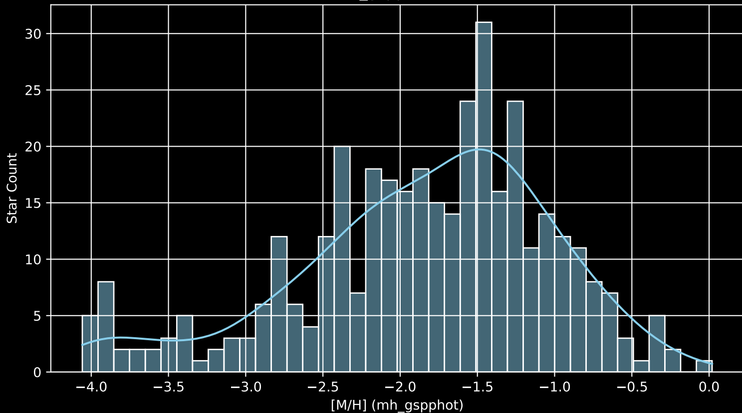
Gaia Stream: [Ylgr [M/H] (mh_gspphot) (n= 371)
