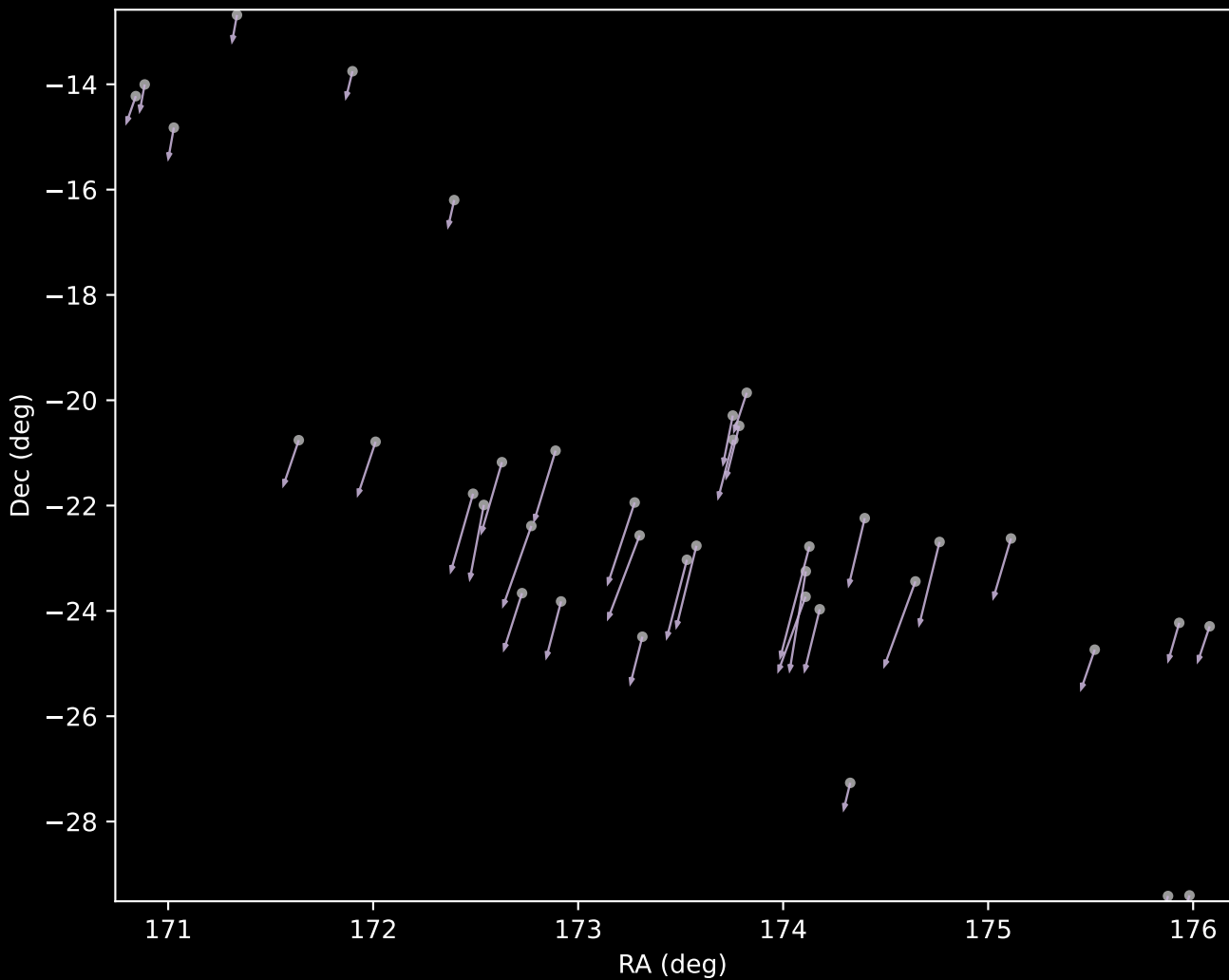
Gaia DR3 Cluster 9 Proper Motion Vectors (n=38)
