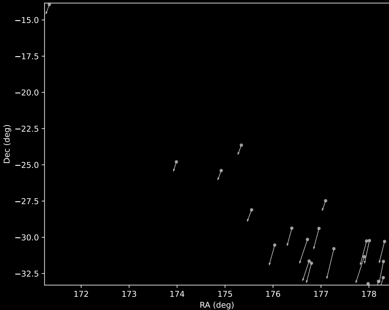
Gaia DR3 Cluster 15 Proper Motion Vectors (n=21)
