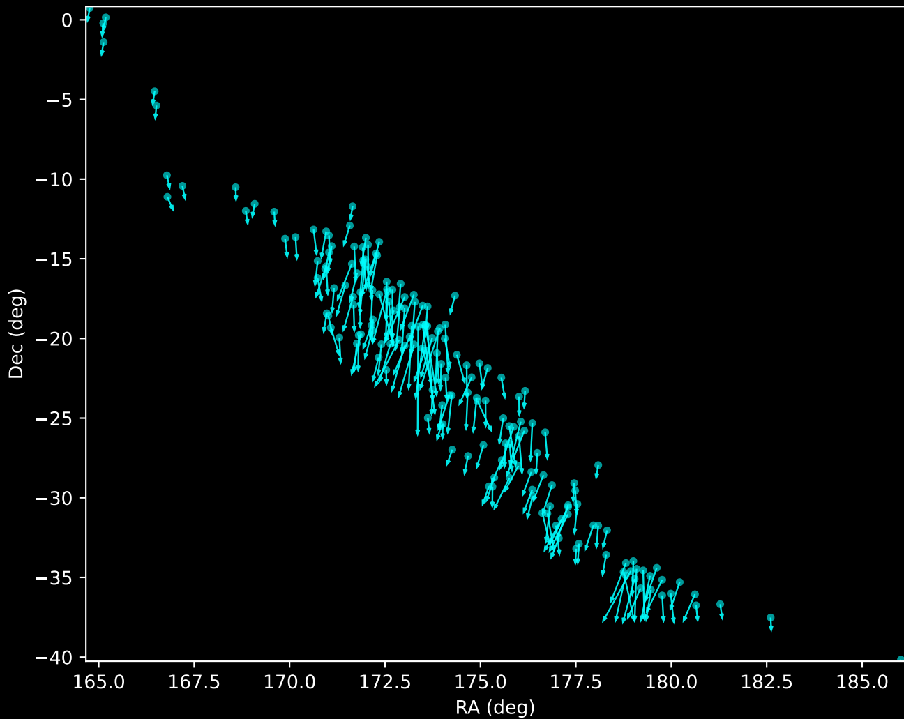
Gaia DR3 HDBSCAN 'Noise' (GD-1 Stream) (n=178)
