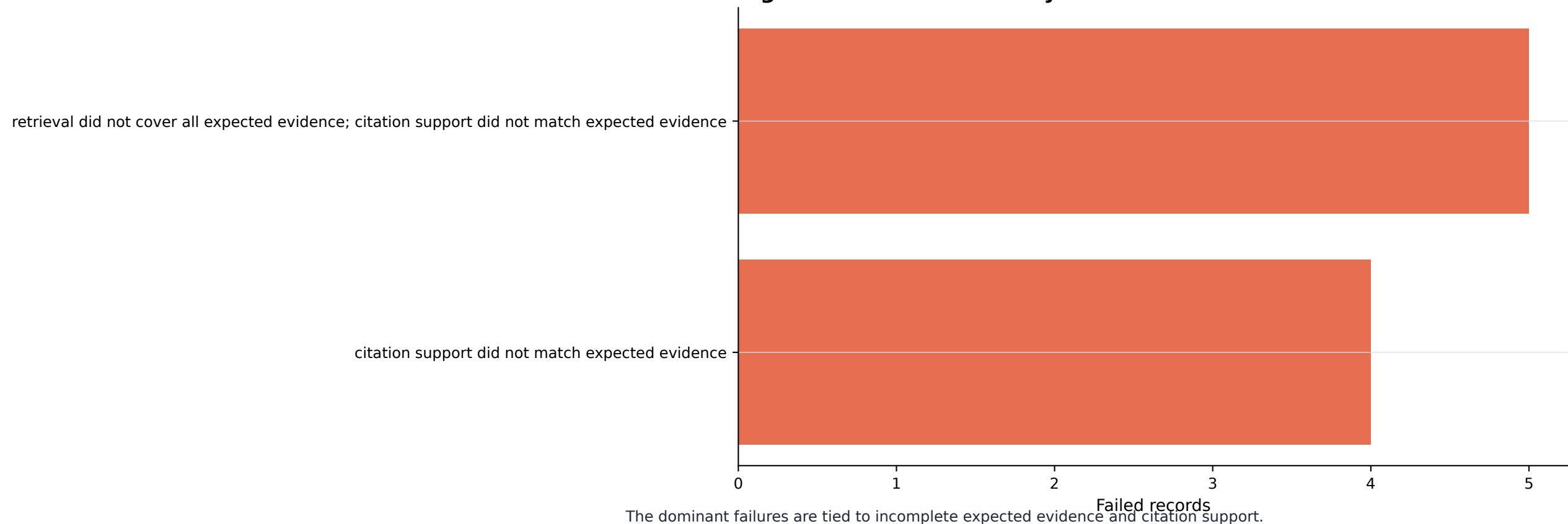
Figure 14. Error taxonomy distribution
