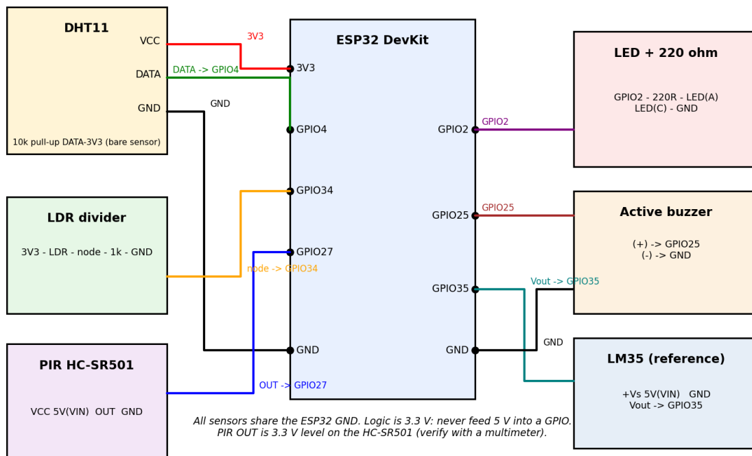
Figure 1(a): Wiring diagram of the node.
