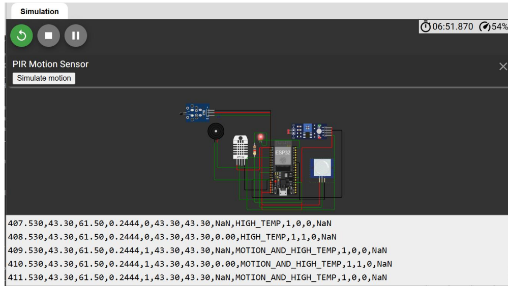
Figure 7: Wokwi simulation with the DHT22 at 43.3 °C and the PIR triggered. The status is MOTION_AND_HIGH_TEMP .
