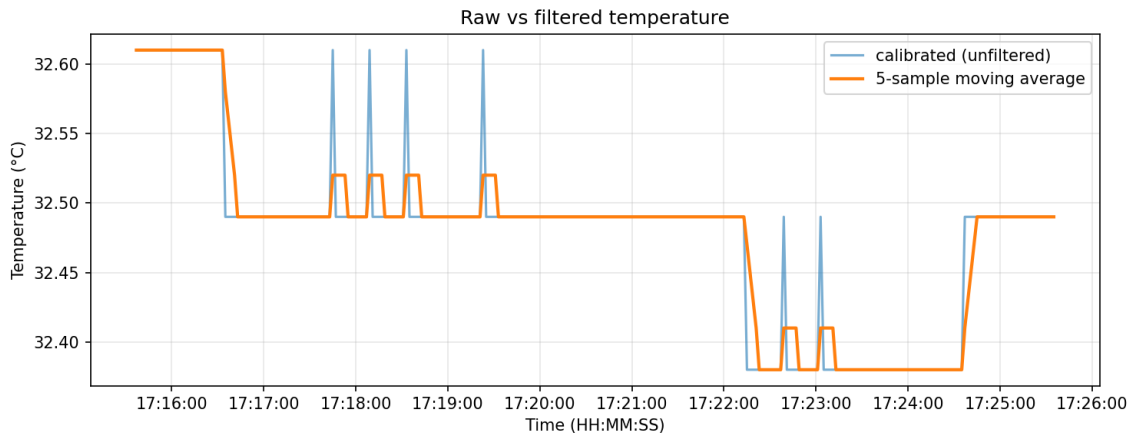
Figure 10: Calibrated temperature and its 5-sample moving average.
