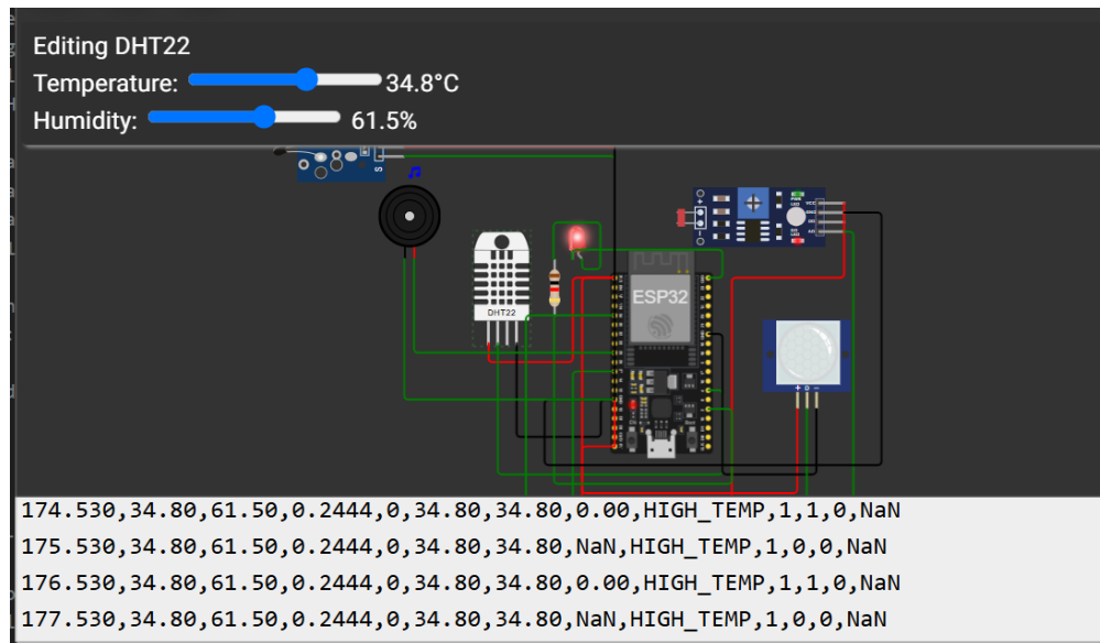
Figure 4: Wokwi simulation with the DHT22 set to 34.8\text{ °C} . The status is still HIGH_TEMP (LED on, buzzer active) because the hysteresis only clears it below 34.5\text{ °C} .
