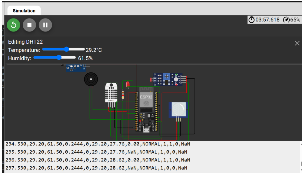
Figure 5: Wokwi simulation after lowering the temperature to 29.2 °C. The status returns to NORMAL, and temp_filt (27.76, then 28.62) is still catching up with temp_cal (29.20), which shows the lag of the 5-sample moving average.
