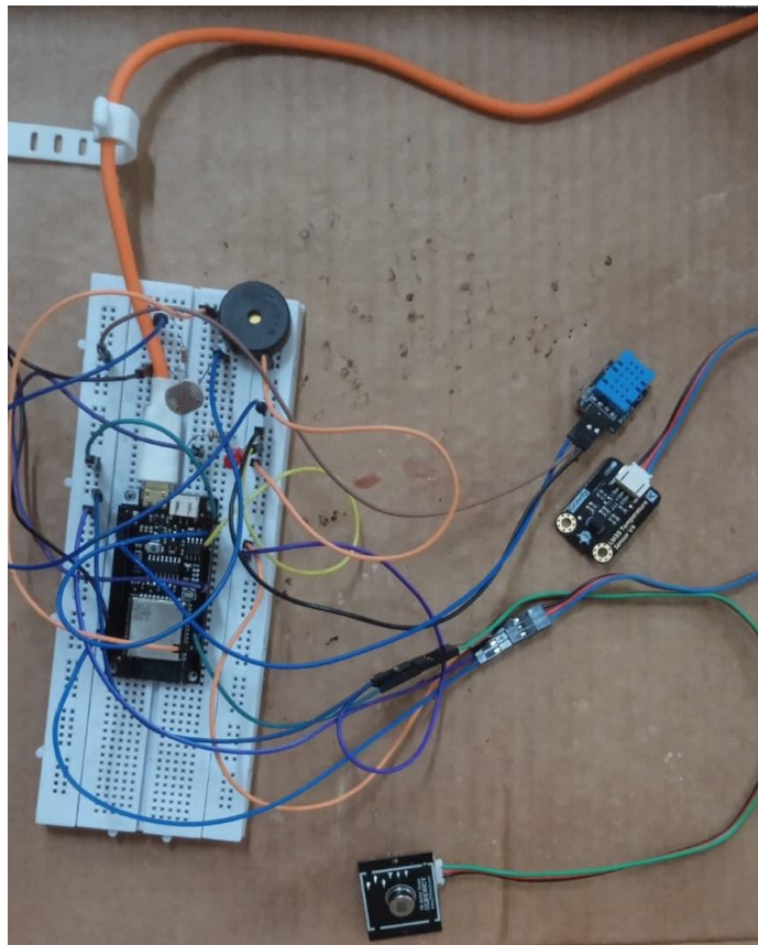
Figure 1(c): The assembled prototype. The ESP32 is on a breadboard with the LDR and buzzer, and the DHT11 and LM35 modules are connected with jumper wires.
