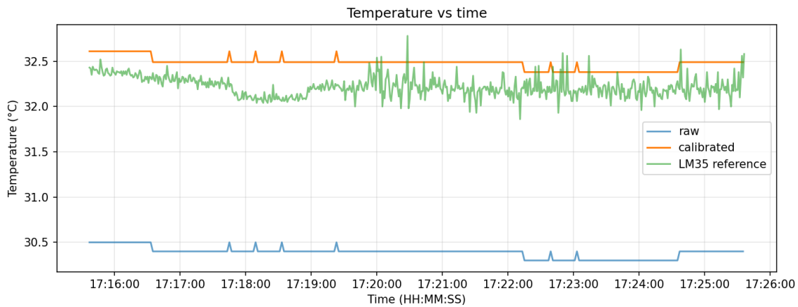
Figure 8: Temperature vs time (raw, calibrated and LM35 reference).
