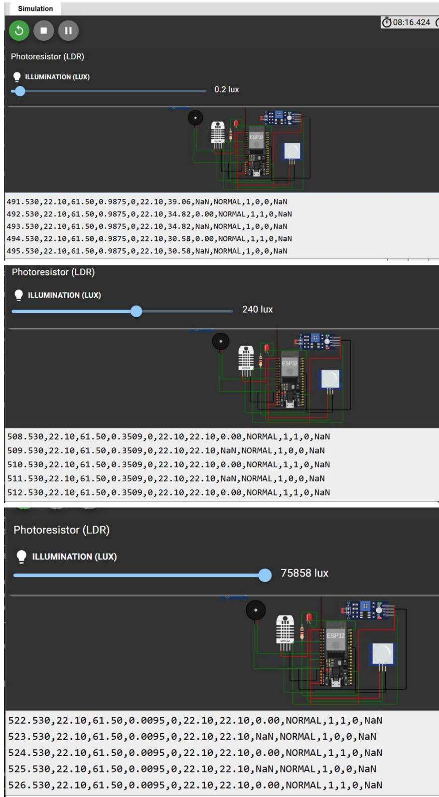
Figure 2: Wokwi simulation of the light channel at 0.2 lux (top, light = 0.9875), 240 lux (middle, 0.3509) and 75858 lux (bottom, 0.0095).
