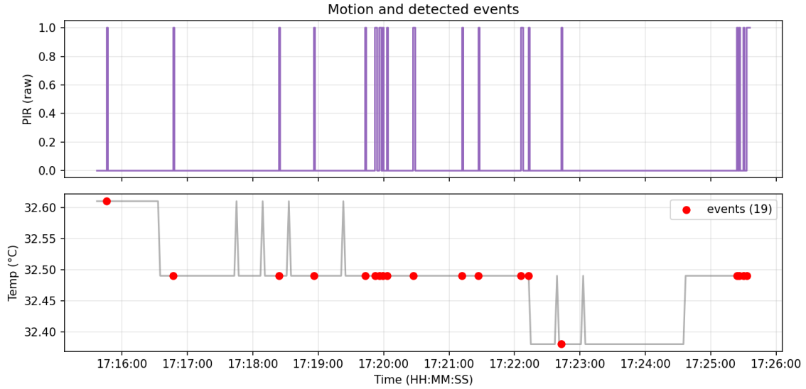
Figure 12: PIR motion and detected events.
