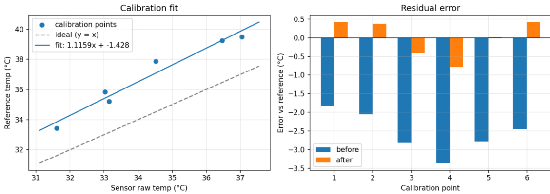
Figure 13: Calibration fit (DHT raw vs LM35) and the residual errors.
