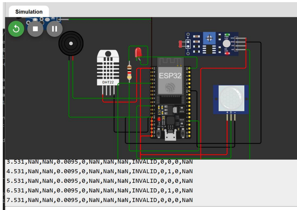
Figure 3: Wokwi simulation with the DHT22 data wire disconnected. The rows are kept as INVALID with valid = 0 and NaN values.
