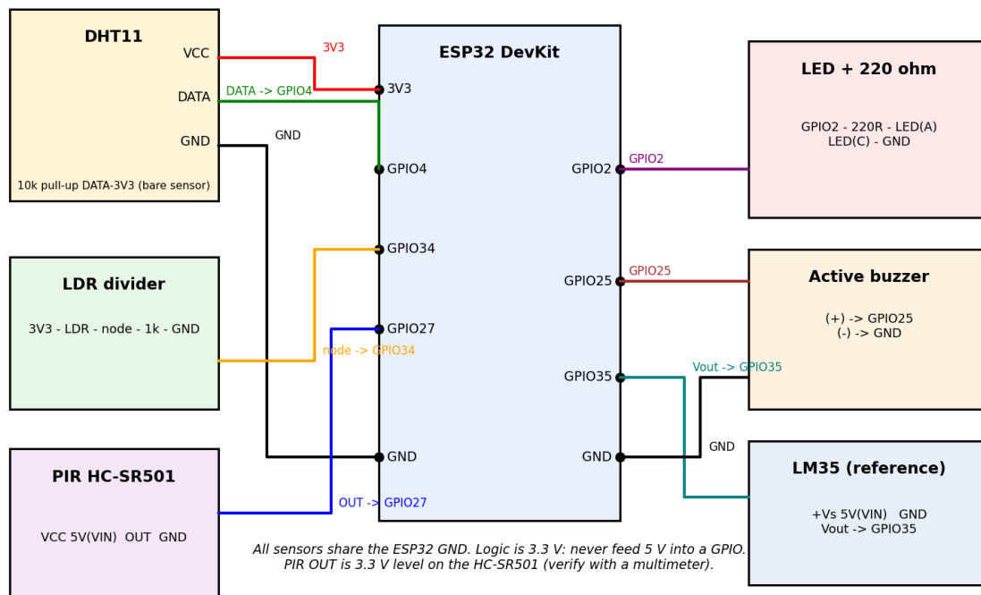
Figure 1(a): Wiring diagram of the node.
