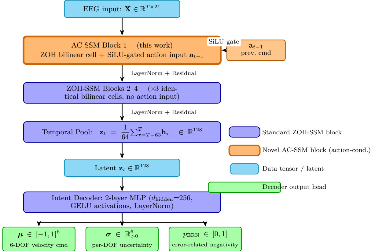
Fig. 2. AC-SSM encoder-decoder architecture (inference path). Orange (thick border): novel action-conditioned Block 1 — the architectural contribution — where the previous motor command \mathbf{a}_{t-1} is injected into the ZOH bilinear recurrence via a SiLU gate. Blue: standard bilinear ZOH-SSM blocks (2–4) with LayerNorm and residual connections; these receive no direct action input. Cyan: input and latent data tensors. Green: three decoder output heads ( \mu , \sigma , p_{ERN} ). The JEPA pretraining path and closed-loop CEM planner are shown in Fig. 1.
