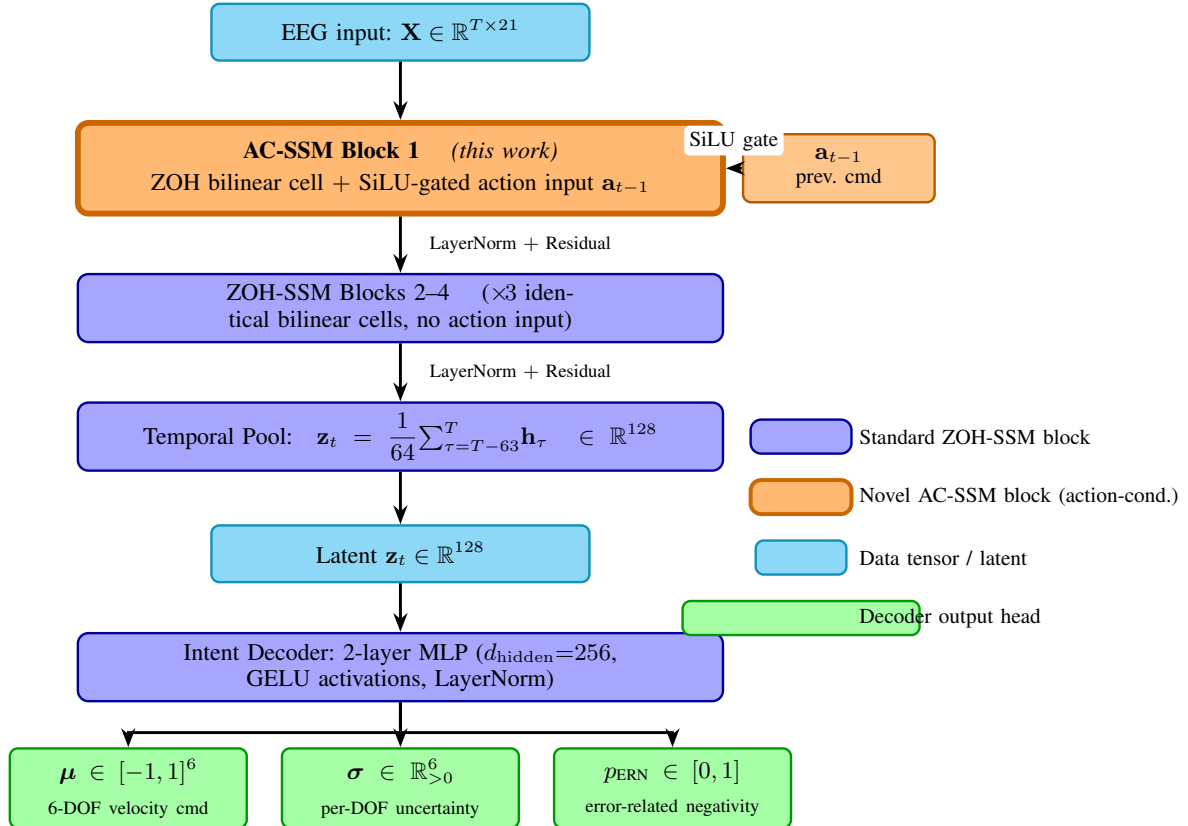
Fig. 2. AC-SSM encoder-decoder architecture (inference path). Orange (thick border): novel action-conditioned Block 1 — the key architectural contribution — where the previous motor command \mathbf{a}_{t-1} is injected into the ZOH bilinear recurrence via a SiLU gate. Blue: standard bilinear ZOH-SSM blocks (2–4) with LayerNorm and residual connections; these receive no direct action input. Cyan: input and latent data tensors. Green: three decoder output heads ( \mu , \sigma , p_{\text{ERN}} ). The JEPa pretraining path and closed-loop CEM planner are shown in Fig. 1.
