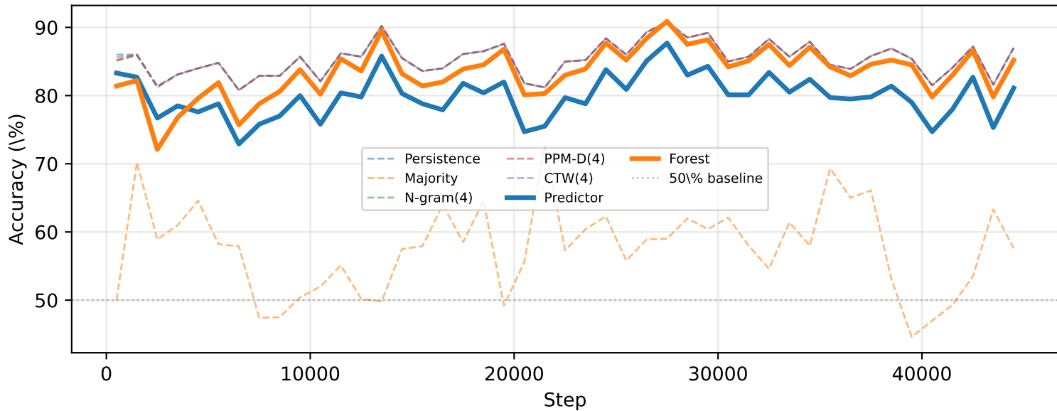
Electricity — rolling accuracy
