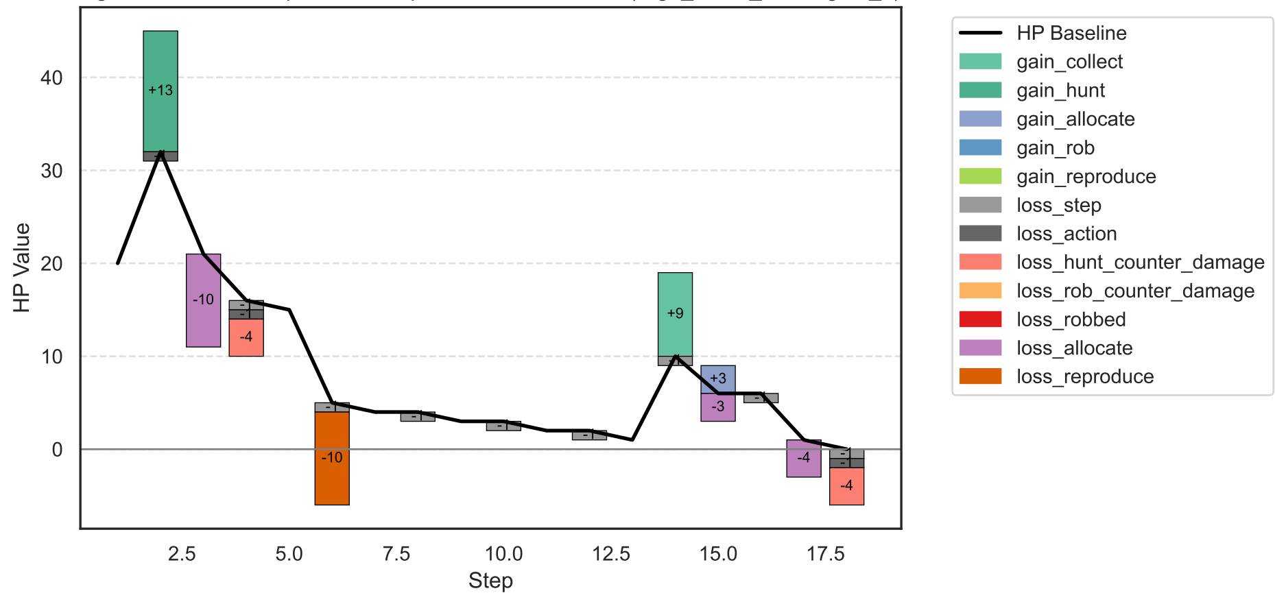
Agent HP Gain/Loss per Time Step with Cause Markers (High_social_cost: agent_1)
