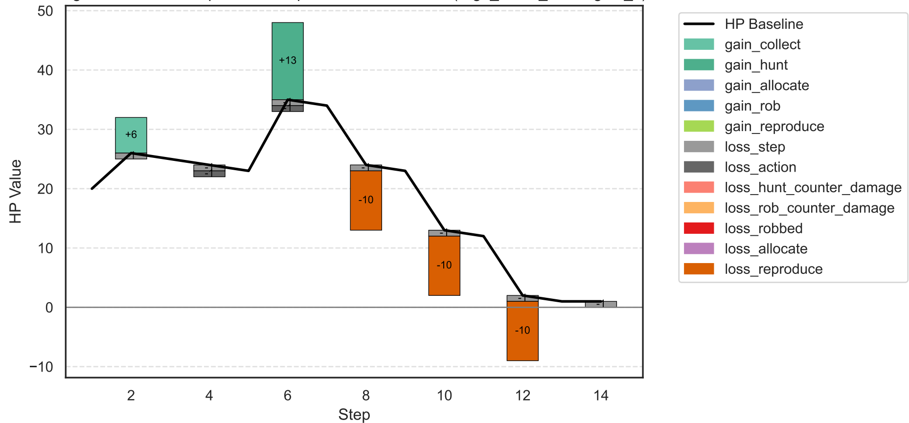
Agent HP Gain/Loss per Time Step with Cause Markers (High_social_cost: agent_7)
