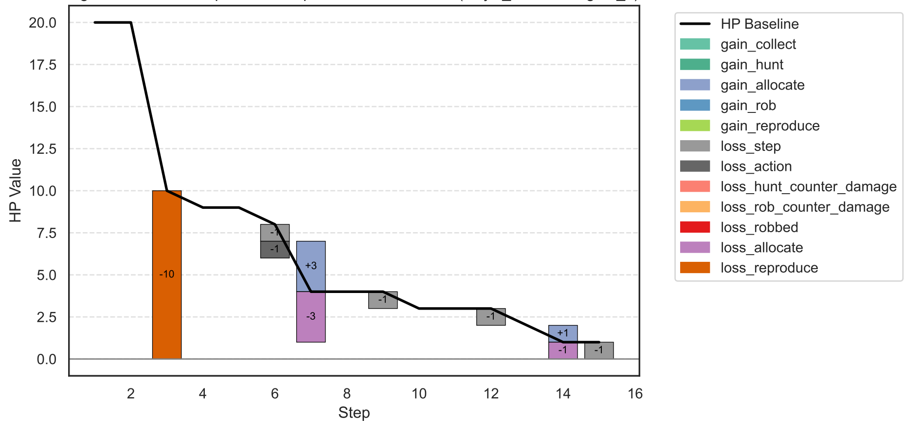
Agent HP Gain/Loss per Time Step with Cause Markers (Major_baseline: agent_5)
