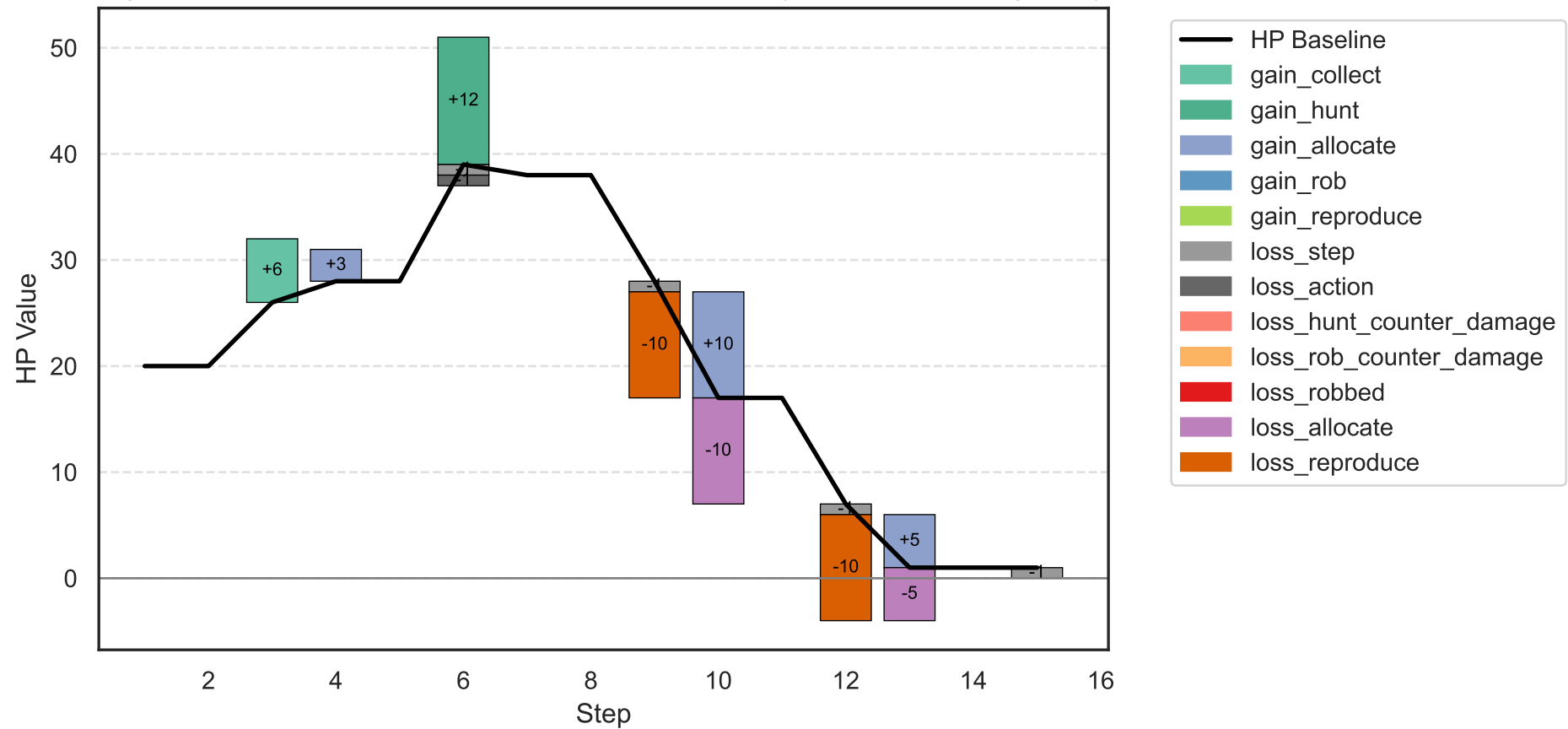
Agent HP Gain/Loss per Time Step with Cause Markers (Moral_invisible: agent_3)
