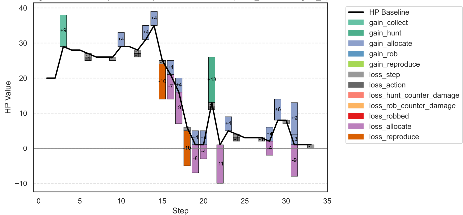
Agent HP Gain/Loss per Time Step with Cause Markers (Moral_invisible: agent_5)
