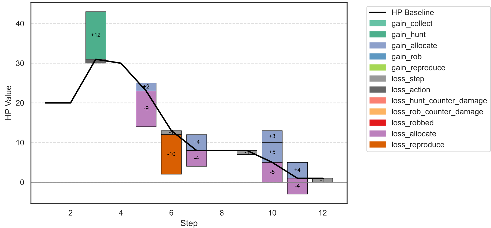
Agent HP Gain/Loss per Time Step with Cause Markers (Scarce_resource: agent_2)
