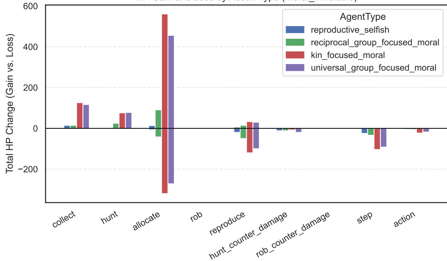
HP Gain and Loss by Action Type (Moral_invisible)
