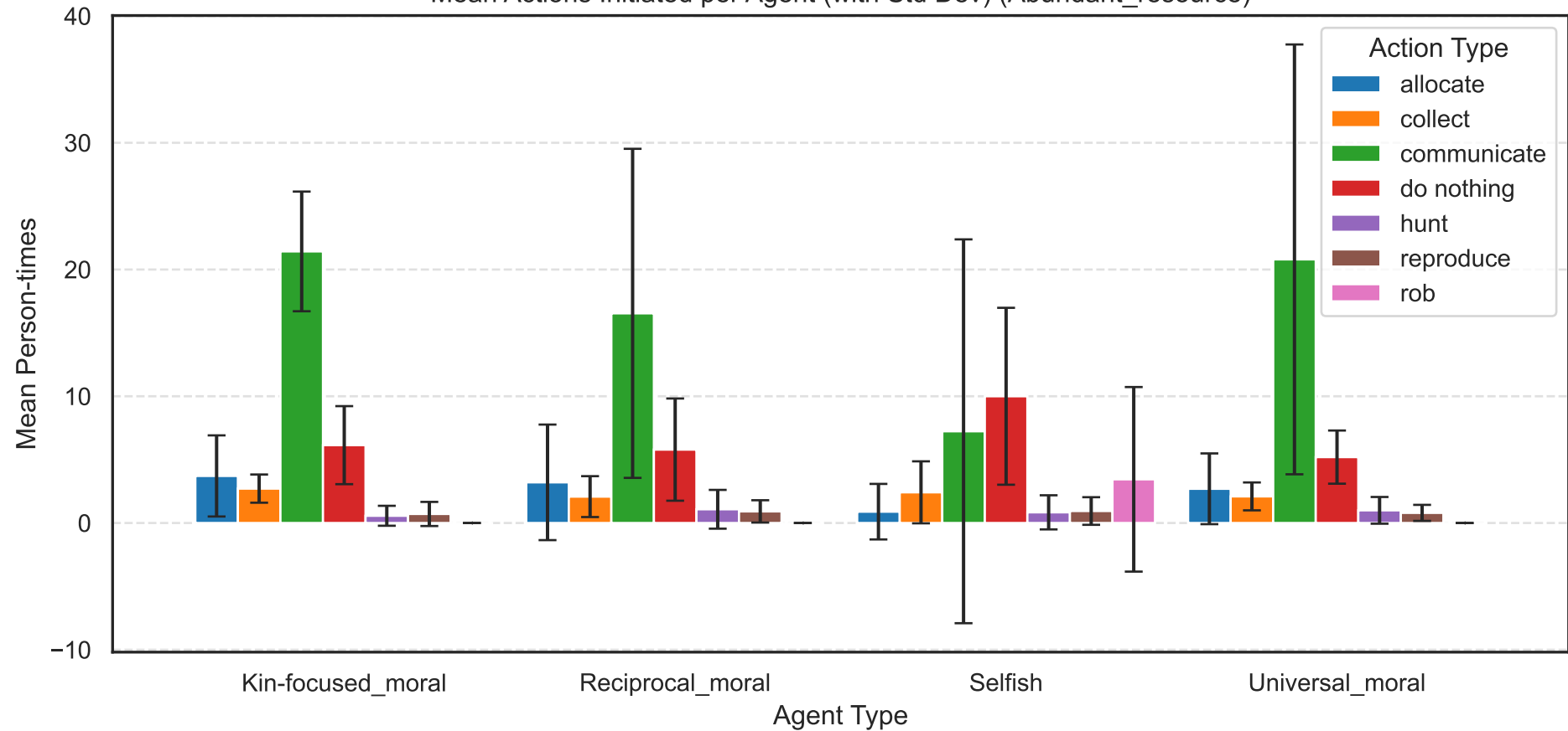
Mean Actions Initiated per Agent (with Std Dev) (Abundant_resource)
