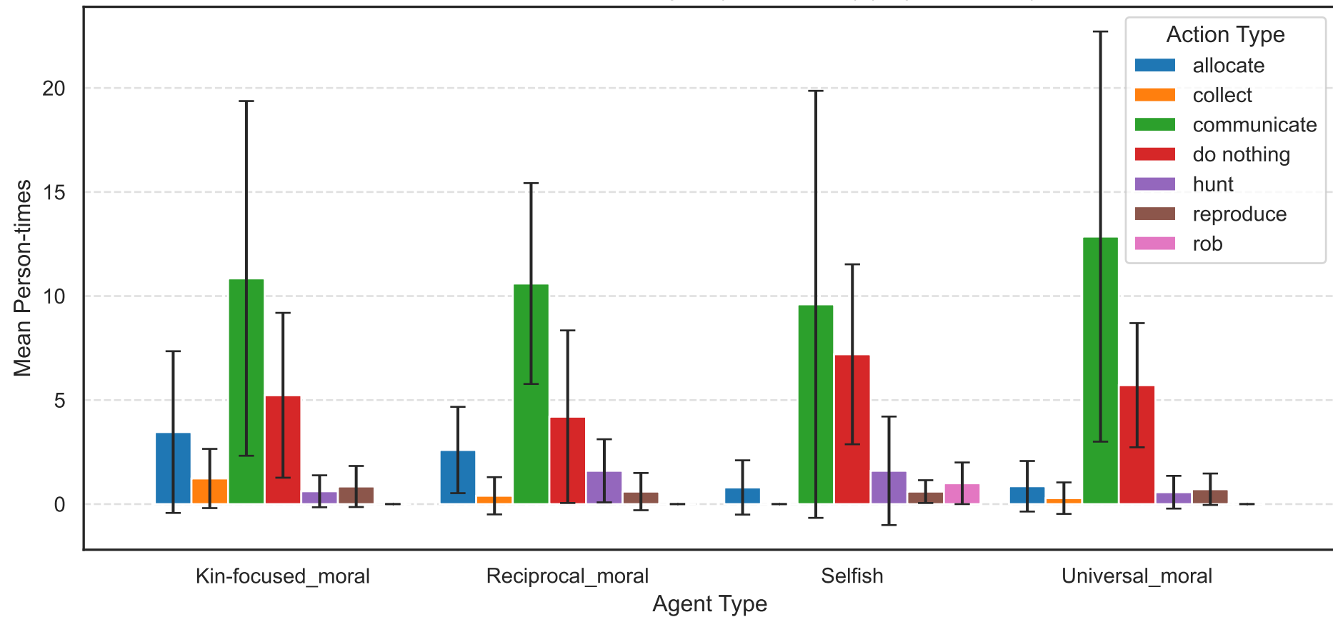
Mean Actions Initiated per Agent (with Std Dev) (Major_baseline)
