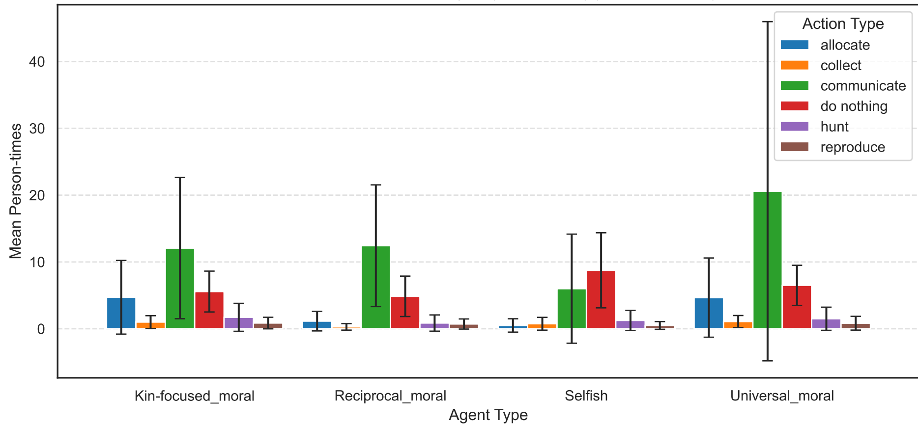
Mean Actions Initiated per Agent (with Std Dev) (Moral_invisible)
