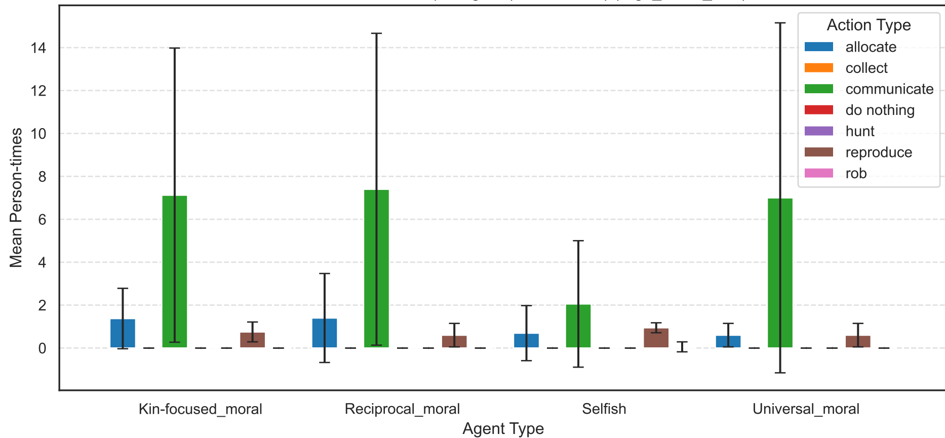
Mean Actions Received per Agent (with Std Dev) (High_social_cost)
