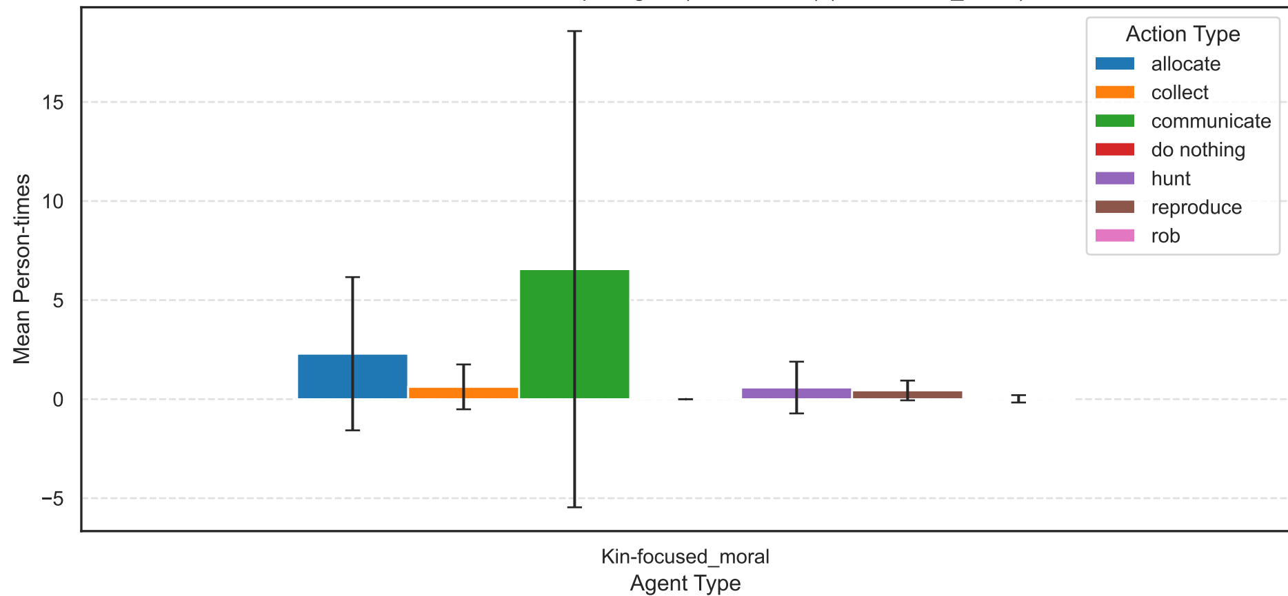
Mean Actions Received per Agent (with Std Dev) (Kin-focused_moral)
