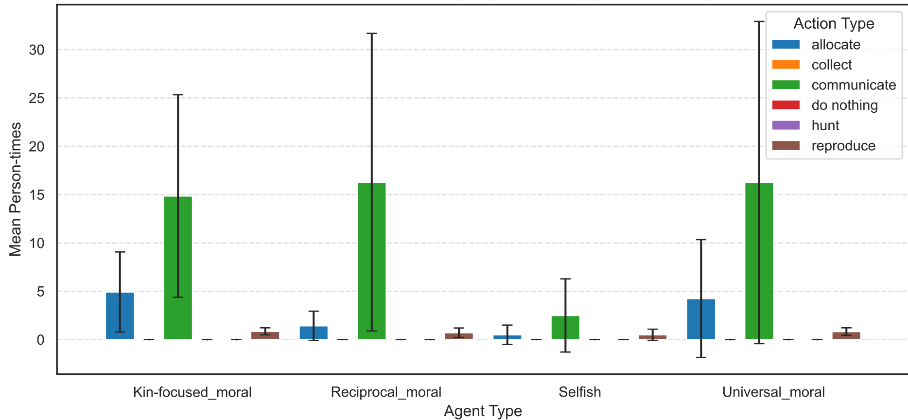
Mean Actions Received per Agent (with Std Dev) (Moral_invisible)
