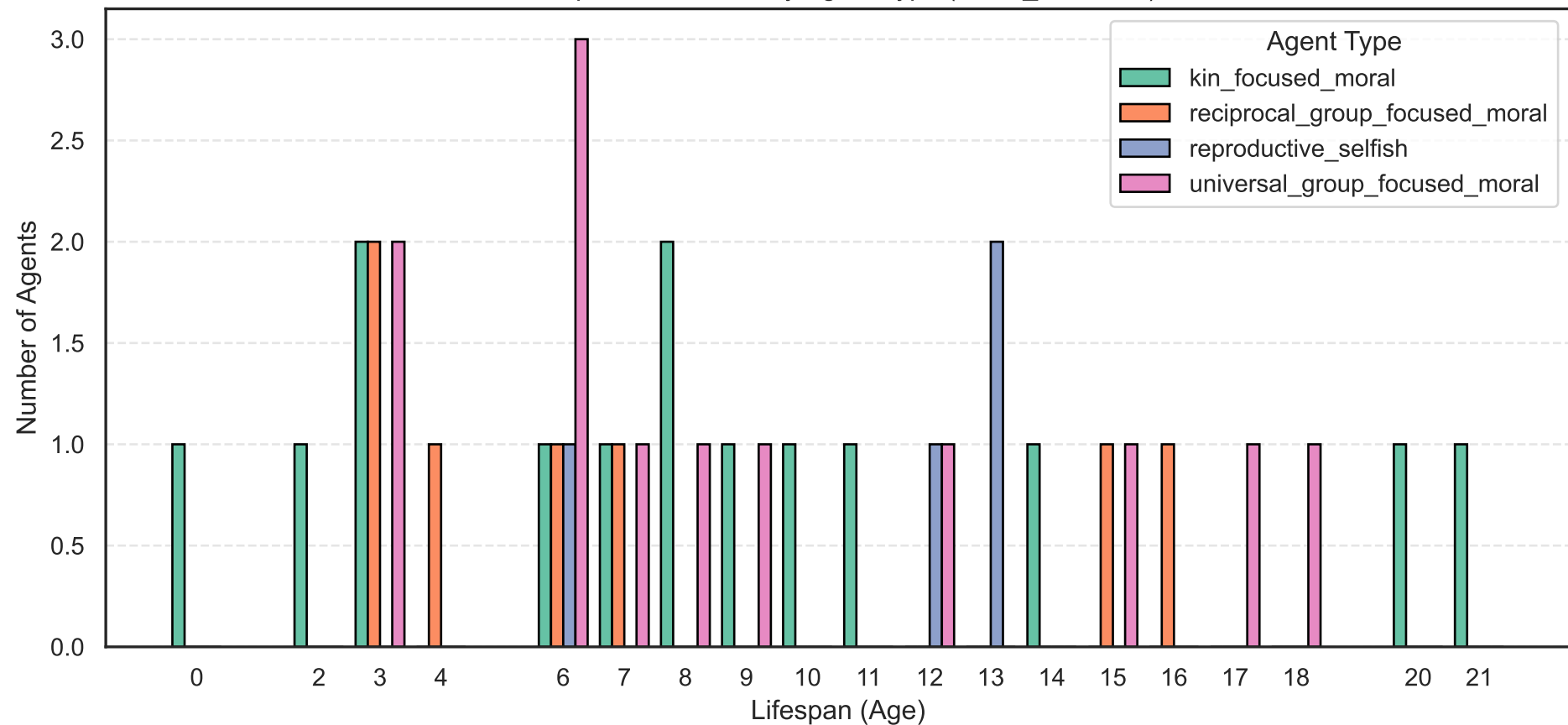
Lifespan Distribution by Agent Type (Moral_invisible)
