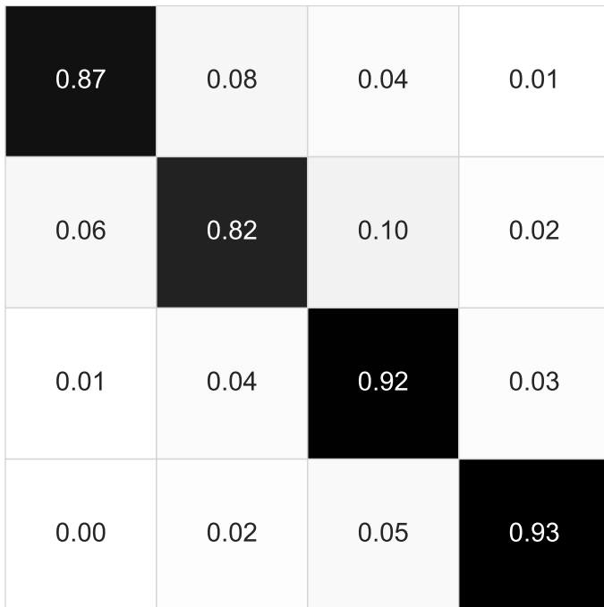
Soft Confusion Matrix (Moral_invisiable)
