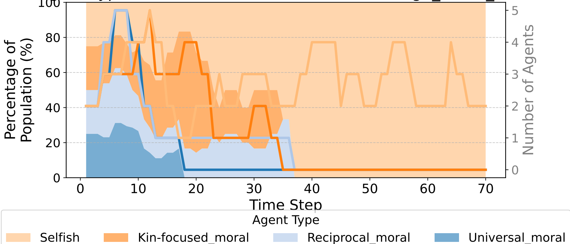
Agent Type Ratio (%) and Count Over Time (High_social_cost)
