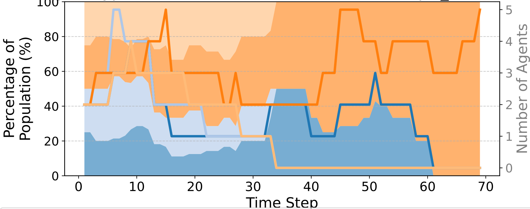
Agent Type Ratio (%) and Count Over Time (Major_baseline)
