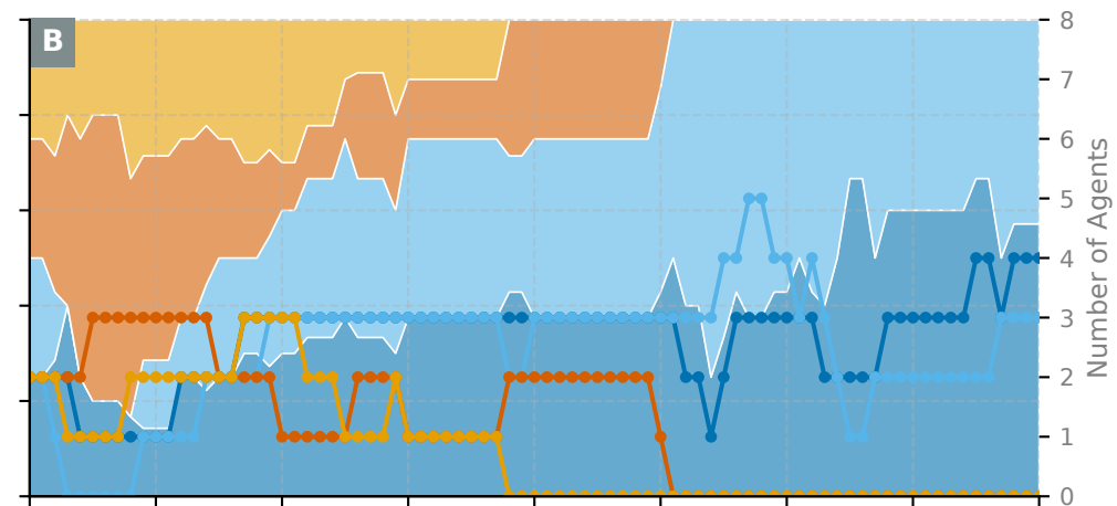
Scarce Resource
