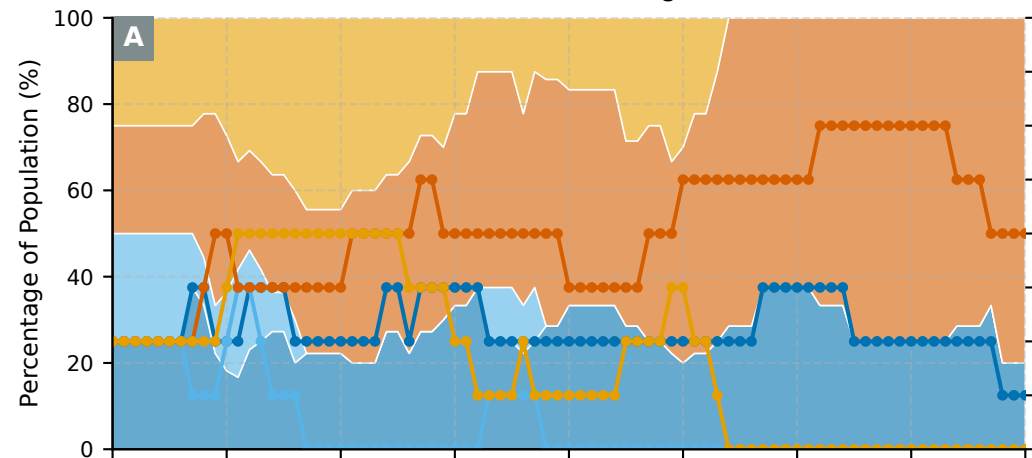
Baseline Setting
