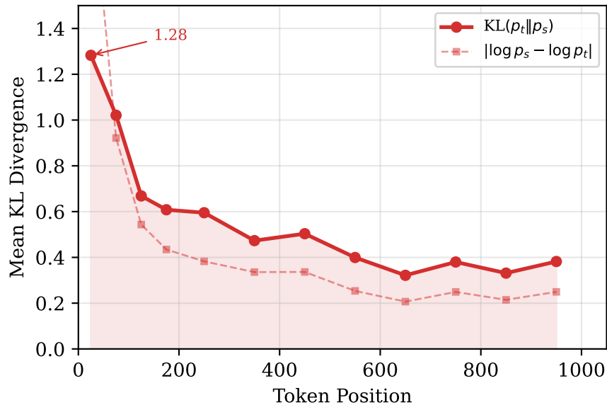
(a) Forward KL(p_t||p_s) by Position
