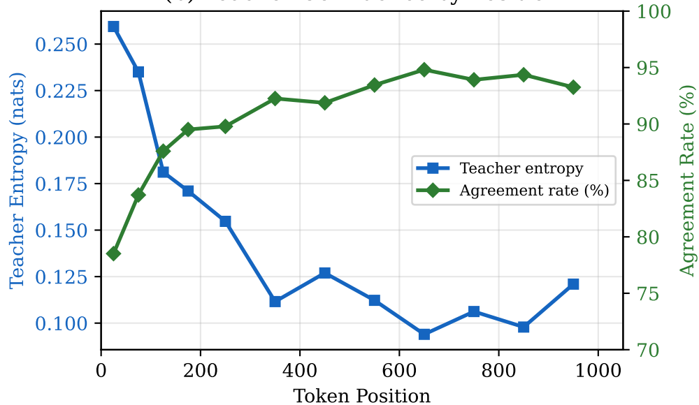
(b) Teacher Confidence by Position
